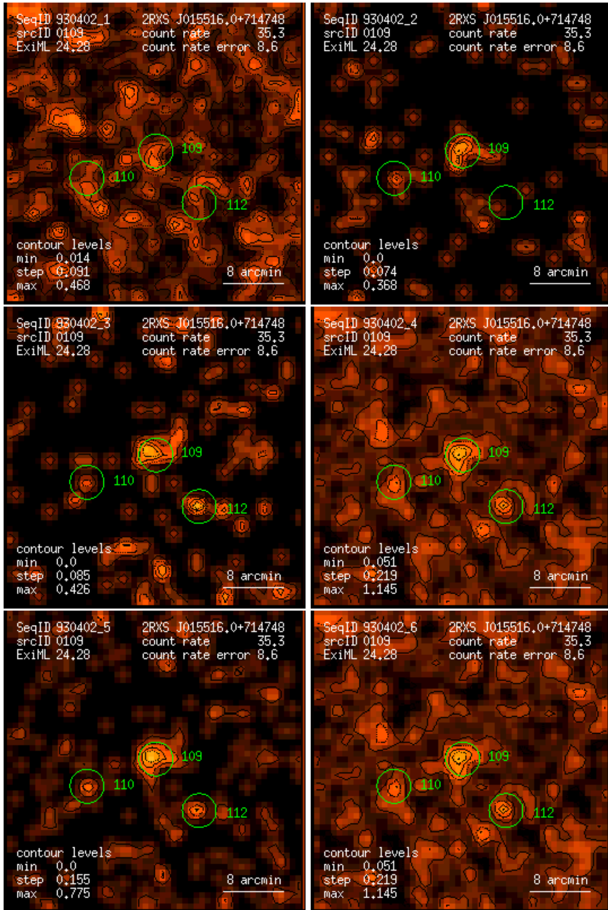
Figure 109: RASS 930402: detection 0109: band rate images, Gaussian filter: (1) PSPC channels 11 – 41, (2) 52 – 90, (3) 91 – 201, (4) 11 – 235, (5) 52 – 201, (6) 11 – 201. Broad band rates in counts/ks. Band rate contour levels in counts/ks/arcmin 2 .
