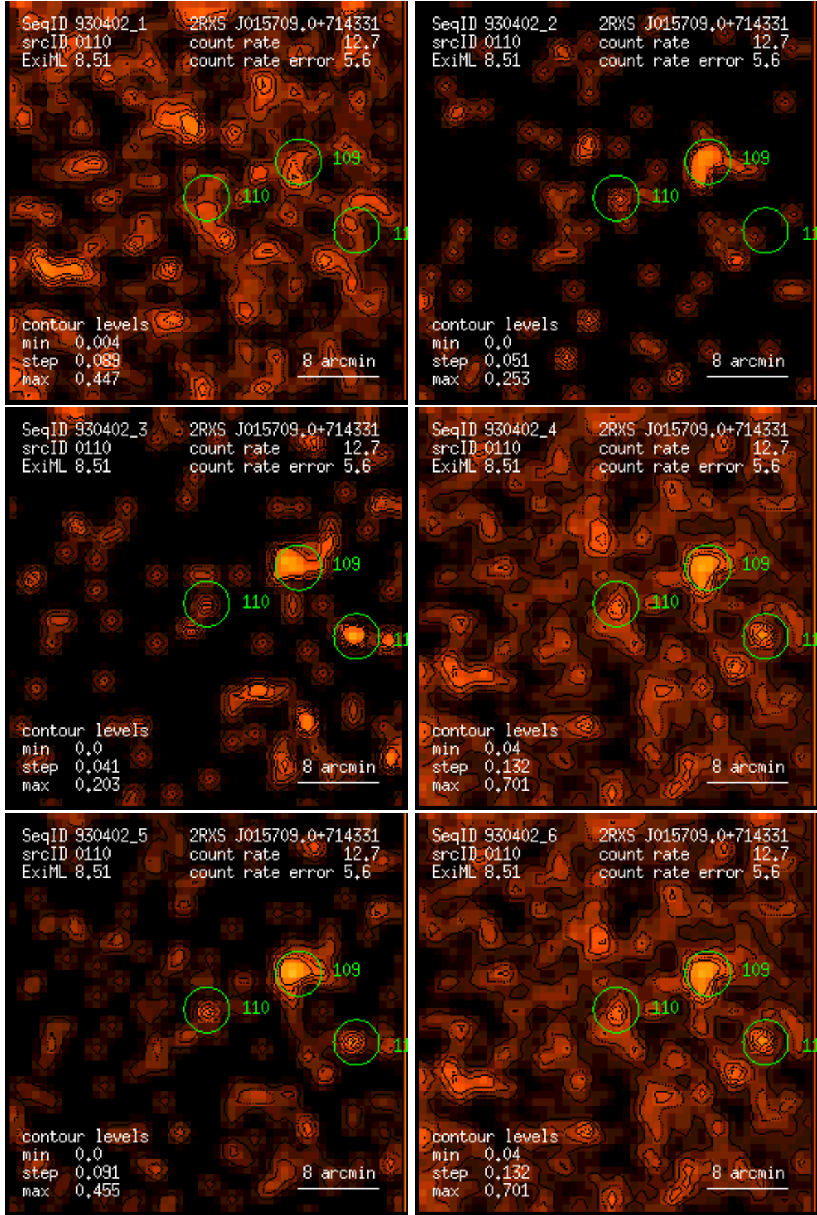
Figure 110: RASS 930402: detection 0110: band rate images, Gaussian filter: (1) PSPC channels 11 – 41, (2) 52 – 90, (3) 91 – 201, (4) 11 – 235, (5) 52 – 201, (6) 11 – 201. Broad band rates in counts/ks. Band rate contour levels in counts/ks/arcmin 2 .
