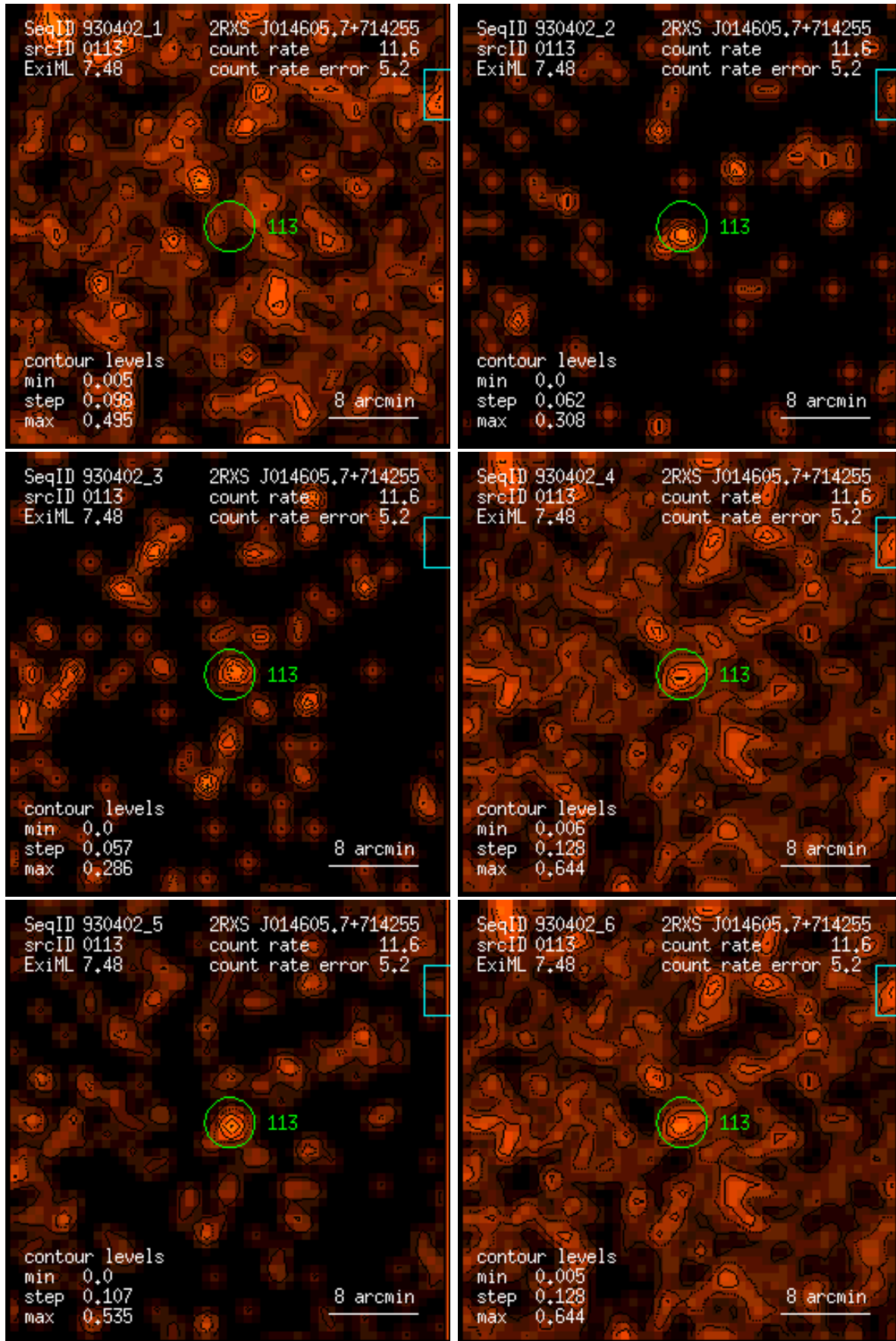
Figure 113: RASS 930402: detection 0113: band rate images, Gaussian filter: (1) PSPC channels 11 – 41, (2) 52 – 90, (3) 91 – 201, (4) 11 – 235, (5) 52 – 201, (6) 11 – 201. Broad band rates in counts/ks. Band rate contour levels in counts/ks/arcmin 2 .
