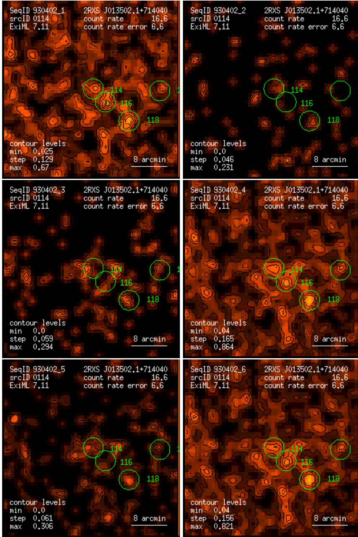
Figure 114: RASS 930402: detection 0114: band rate images, Gaussian filter: (1) PSPC channels 11 – 41, (2) 52 – 90, (3) 91 – 201, (4) 11 – 235, (5) 52 – 201, (6) 11 – 201. Broad band rates in counts/ks. Band rate contour levels in counts/ks/arcmin 2 .
