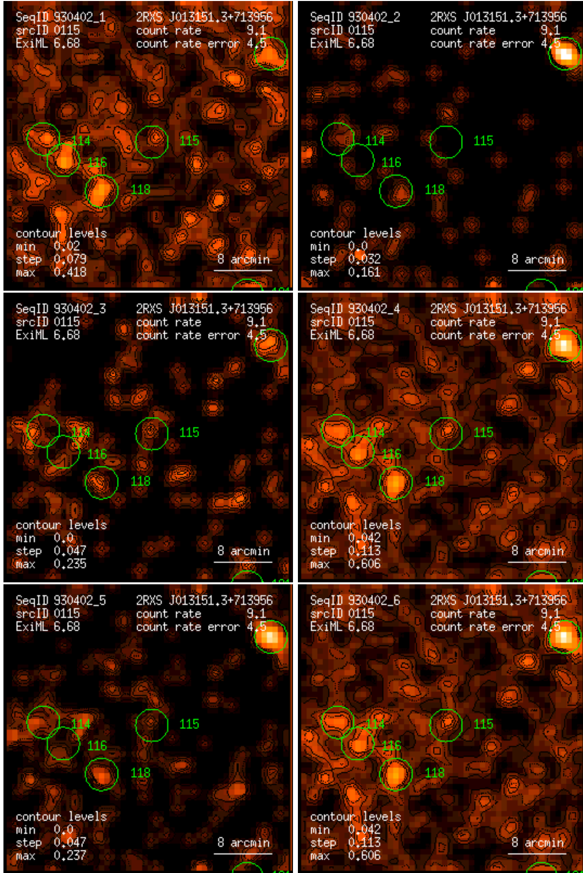
Figure 115: RASS 930402: detection 0115: band rate images, Gaussian filter: (1) PSPC channels 11 – 41, (2) 52 – 90, (3) 91 – 201, (4) 11 – 235, (5) 52 – 201, (6) 11 – 201. Broad band rates in counts/ks. Band rate contour levels in counts/ks/arcmin 2 .
