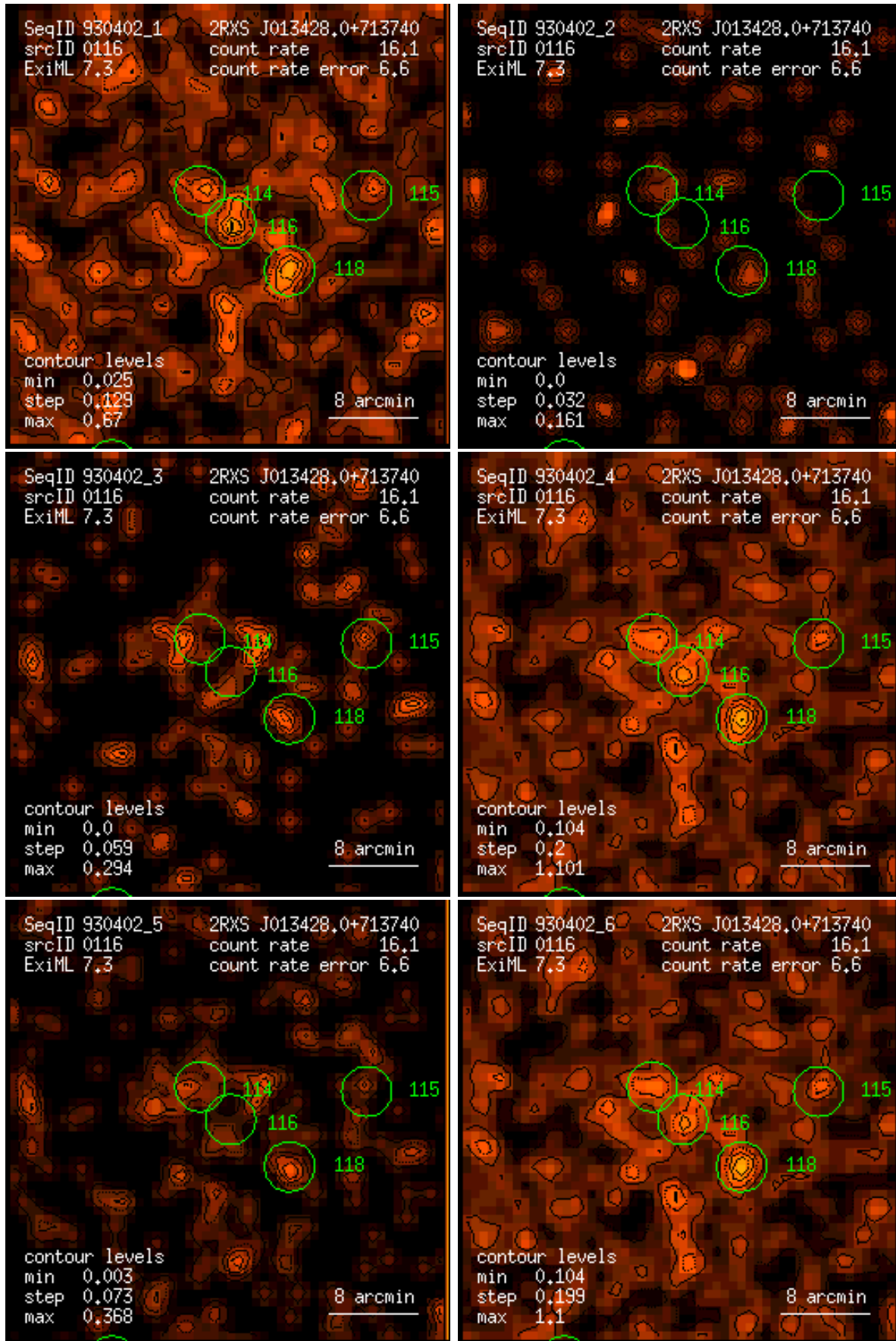
Figure 116: RASS 930402: detection 0116: band rate images, Gaussian filter: (1) PSPC channels 11 – 41, (2) 52 – 90, (3) 91 – 201, (4) 11 – 235, (5) 52 – 201, (6) 11 – 201. Broad band rates in counts/ks. Band rate contour levels in counts/ks/arcmin 2 .
