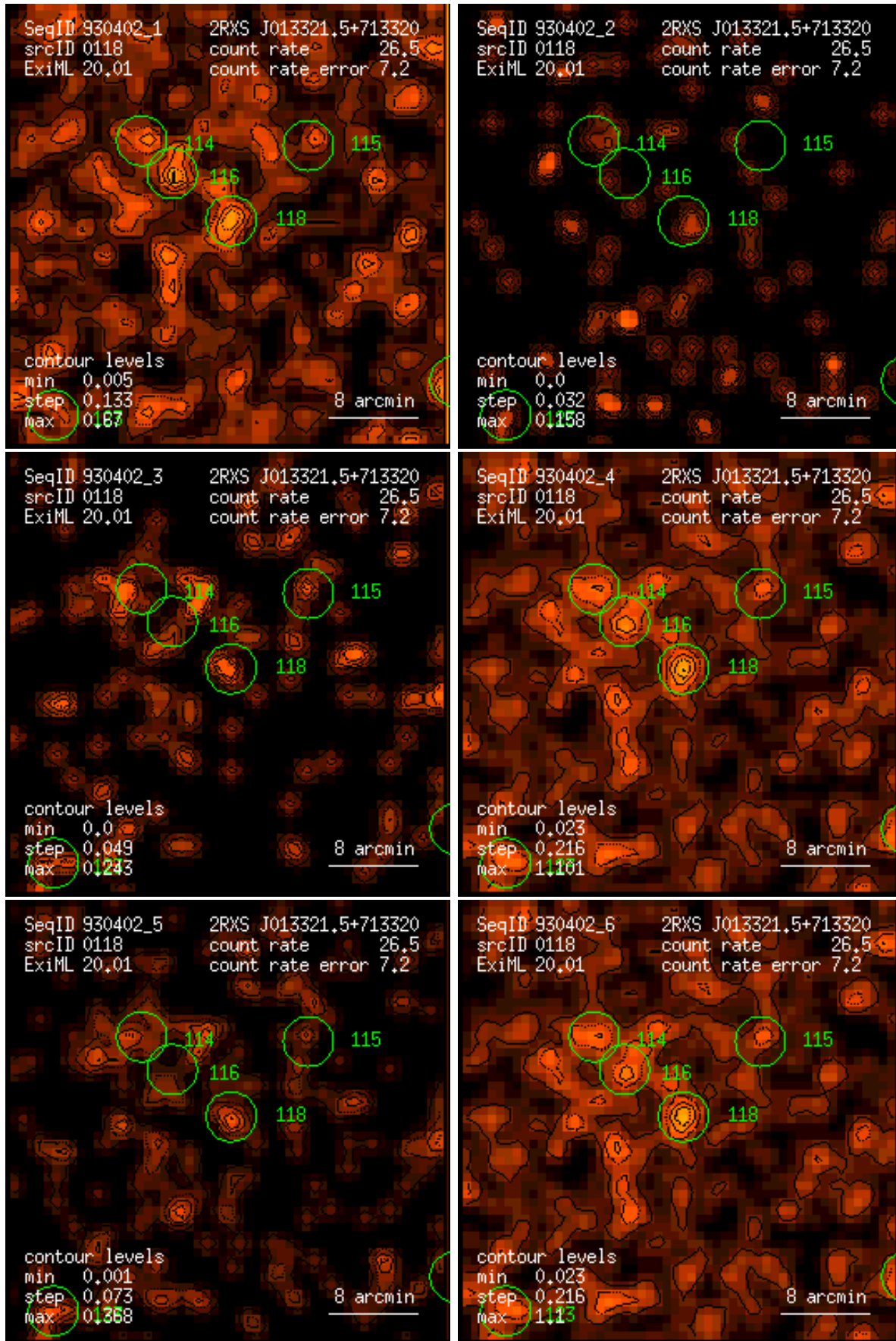
Figure 118: RASS 930402: detection 0118: band rate images, Gaussian filter: (1) PSPC channels 11 – 41, (2) 52 – 90, (3) 91 – 201, (4) 11 – 235, (5) 52 – 201, (6) 11 – 201. Broad band rates in counts/ks. Band rate contour levels in counts/ks/arcmin 2 .
