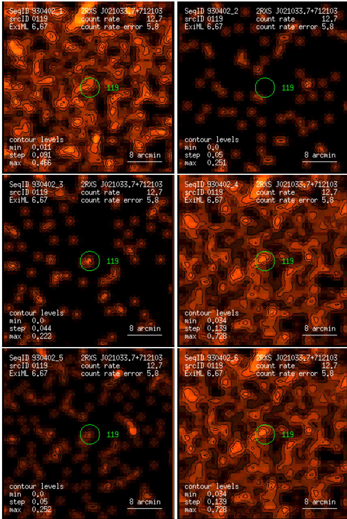
Figure 119: RASS 930402: detection 0119: band rate images, Gaussian filter: (1) PSPC channels 11 – 41, (2) 52 – 90, (3) 91 – 201, (4) 11 – 235, (5) 52 – 201, (6) 11 – 201. Broad band rates in counts/ks. Band rate contour levels in counts/ks/arcmin 2 .
