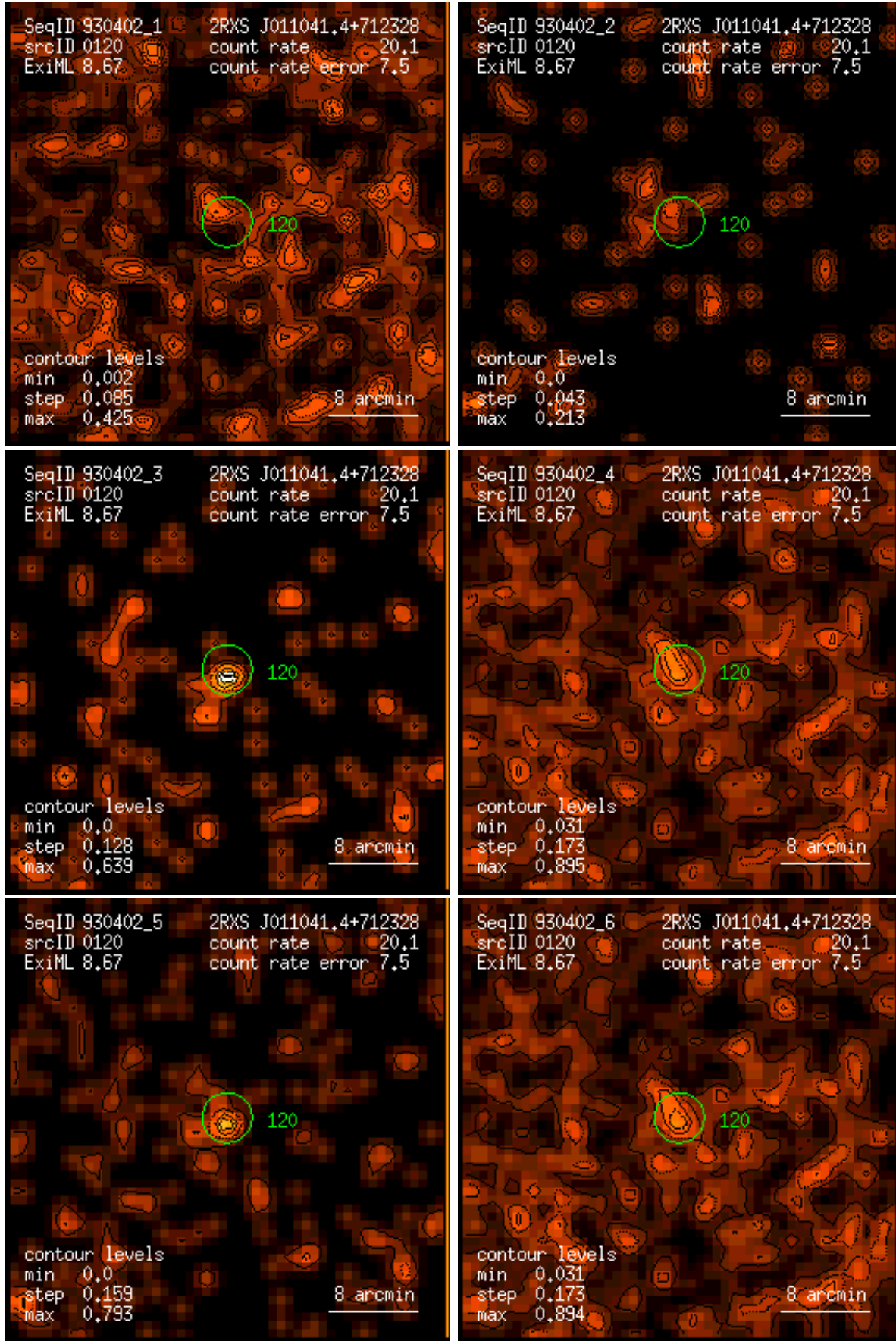
Figure 120: RASS 930402: detection 0120: band rate images, Gaussian filter: (1) PSPC channels 11 – 41, (2) 52 – 90, (3) 91 – 201, (4) 11 – 235, (5) 52 – 201, (6) 11 – 201. Broad band rates in counts/ks. Band rate contour levels in counts/ks/arcmin 2 .
