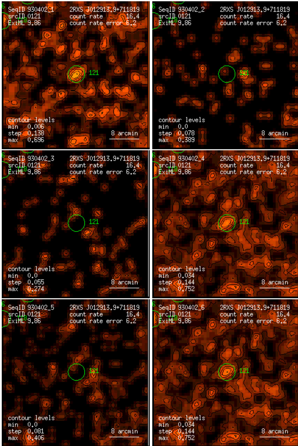
Figure 121: RASS 930402: detection 0121: band rate images, Gaussian filter: (1) PSPC channels 11 – 41, (2) 52 – 90, (3) 91 – 201, (4) 11 – 235, (5) 52 – 201, (6) 11 – 201. Broad band rates in counts/ks. Band rate contour levels in counts/ks/arcmin 2 .
