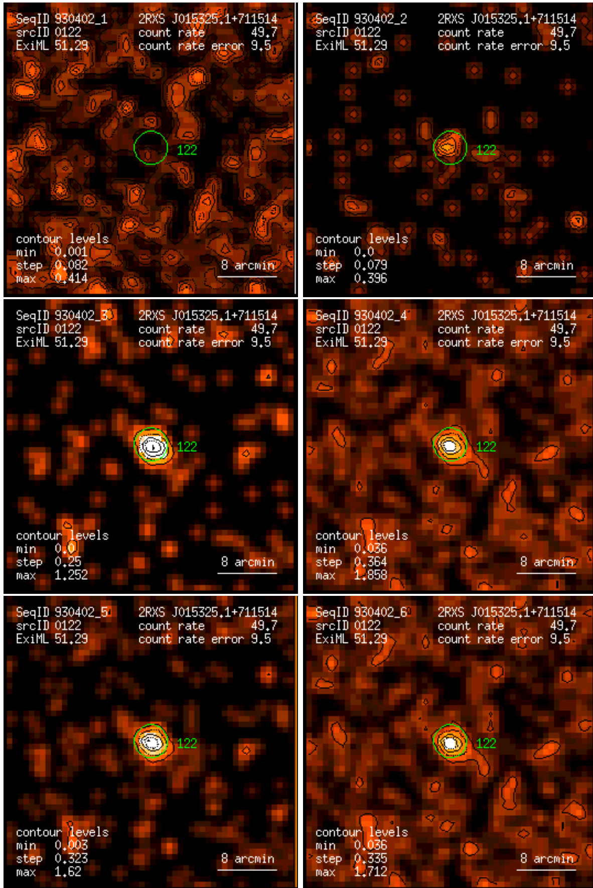
Figure 122: RASS 930402: detection 0122: band rate images, Gaussian filter: (1) PSPC channels 11 – 41, (2) 52 – 90, (3) 91 – 201, (4) 11 – 235, (5) 52 – 201, (6) 11 – 201. Broad band rates in counts/ks. Band rate contour levels in counts/ks/arcmin 2 .
