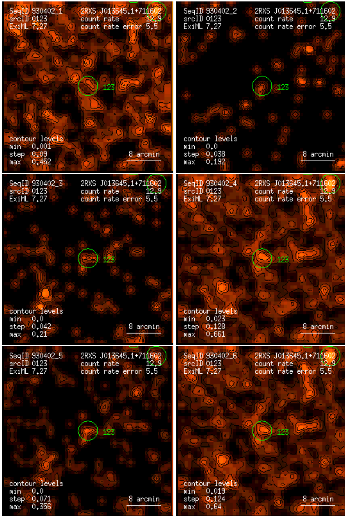
Figure 123: RASS 930402: detection 0123: band rate images, Gaussian filter: (1) PSPC channels 11 – 41, (2) 52 – 90, (3) 91 – 201, (4) 11 – 235, (5) 52 – 201, (6) 11 – 201. Broad band rates in counts/ks. Band rate contour levels in counts/ks/arcmin 2 .
