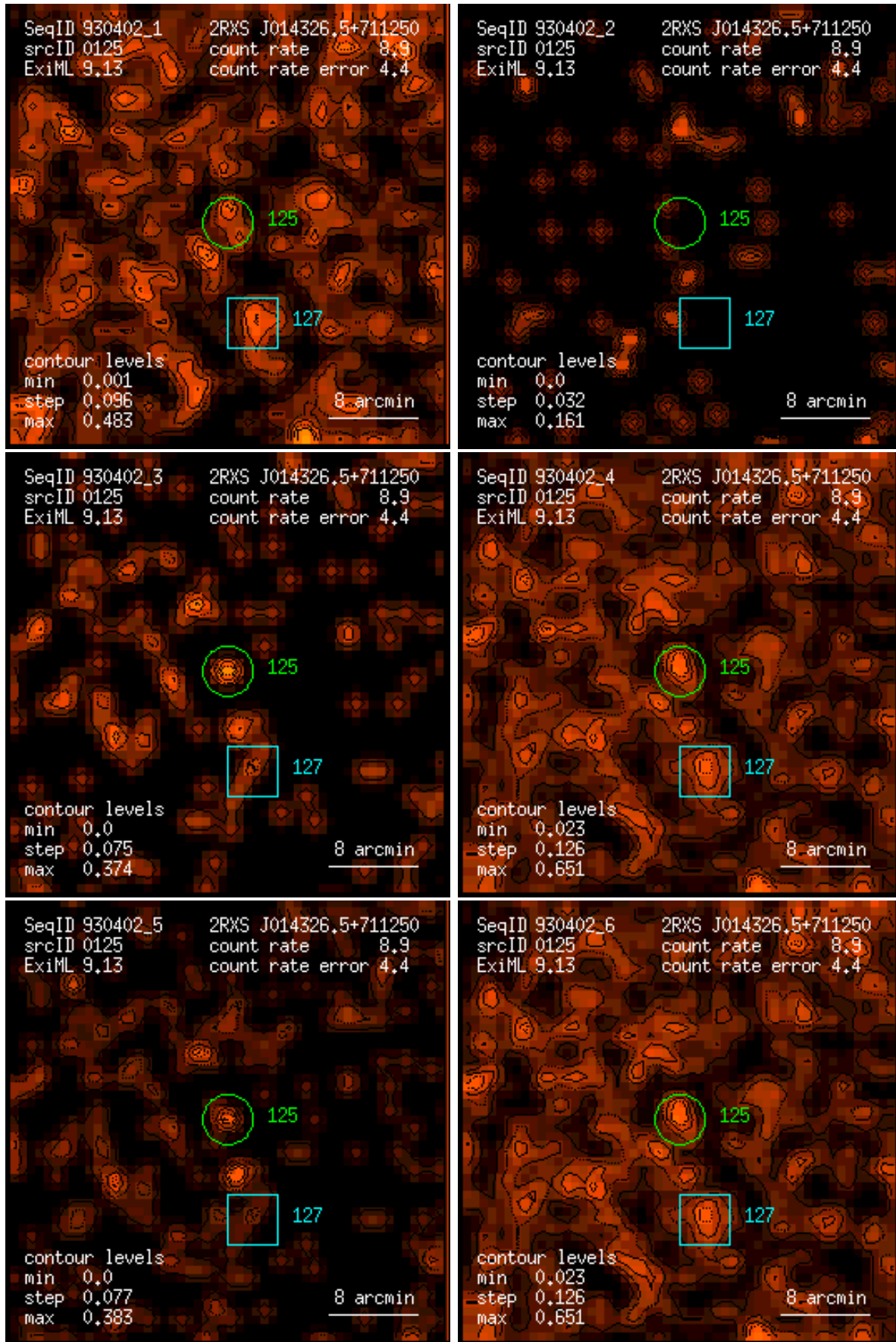
Figure 125: RASS 930402: detection 0125: band rate images, Gaussian filter: (1) PSPC channels 11 – 41, (2) 52 – 90, (3) 91 – 201, (4) 11 – 235, (5) 52 – 201, (6) 11 – 201. Broad band rates in counts/ks. Band rate contour levels in counts/ks/arcmin 2 .
