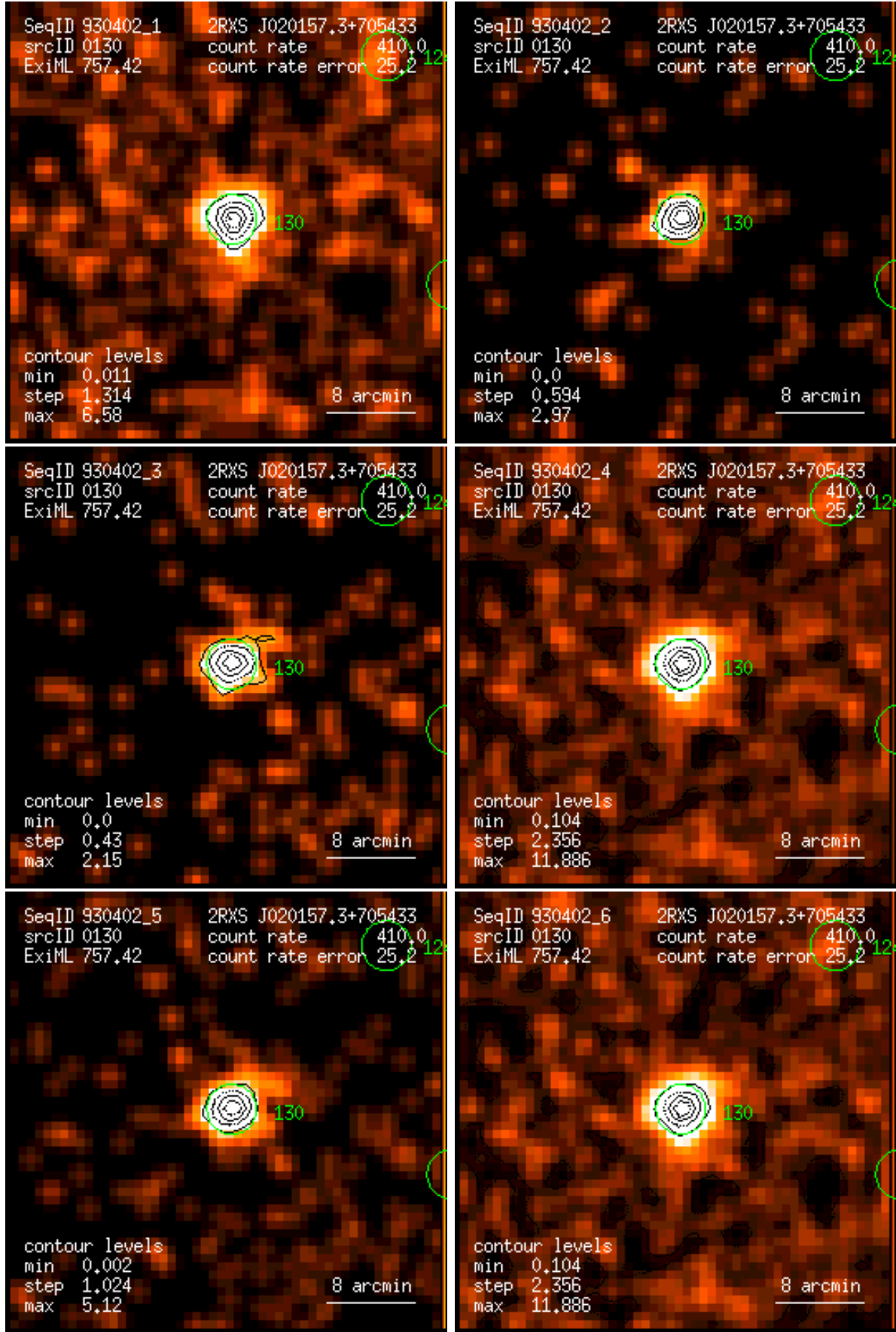
Figure 130: RASS 930402: detection 0130: band rate images, Gaussian filter: (1) PSPC channels 11 – 41, (2) 52 – 90, (3) 91 – 201, (4) 11 – 235, (5) 52 – 201, (6) 11 – 201. Broad band rates in counts/ks. Band rate contour levels in counts/ks/arcmin 2 .
