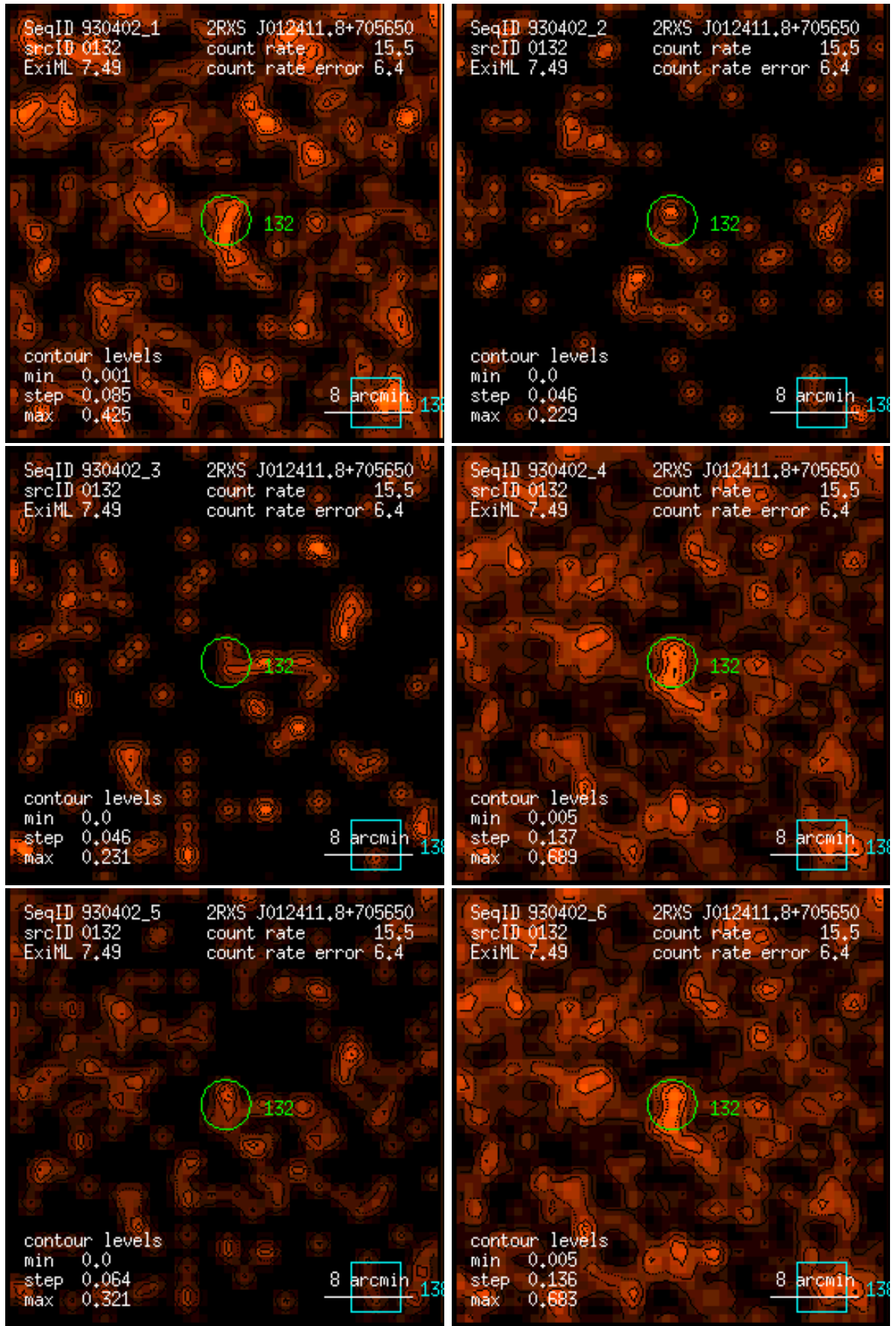
Figure 132: RASS 930402: detection 0132: band rate images, Gaussian filter: (1) PSPC channels 11 – 41, (2) 52 – 90, (3) 91 – 201, (4) 11 – 235, (5) 52 – 201, (6) 11 – 201. Broad band rates in counts/ks. Band rate contour levels in counts/ks/arcmin 2 .
