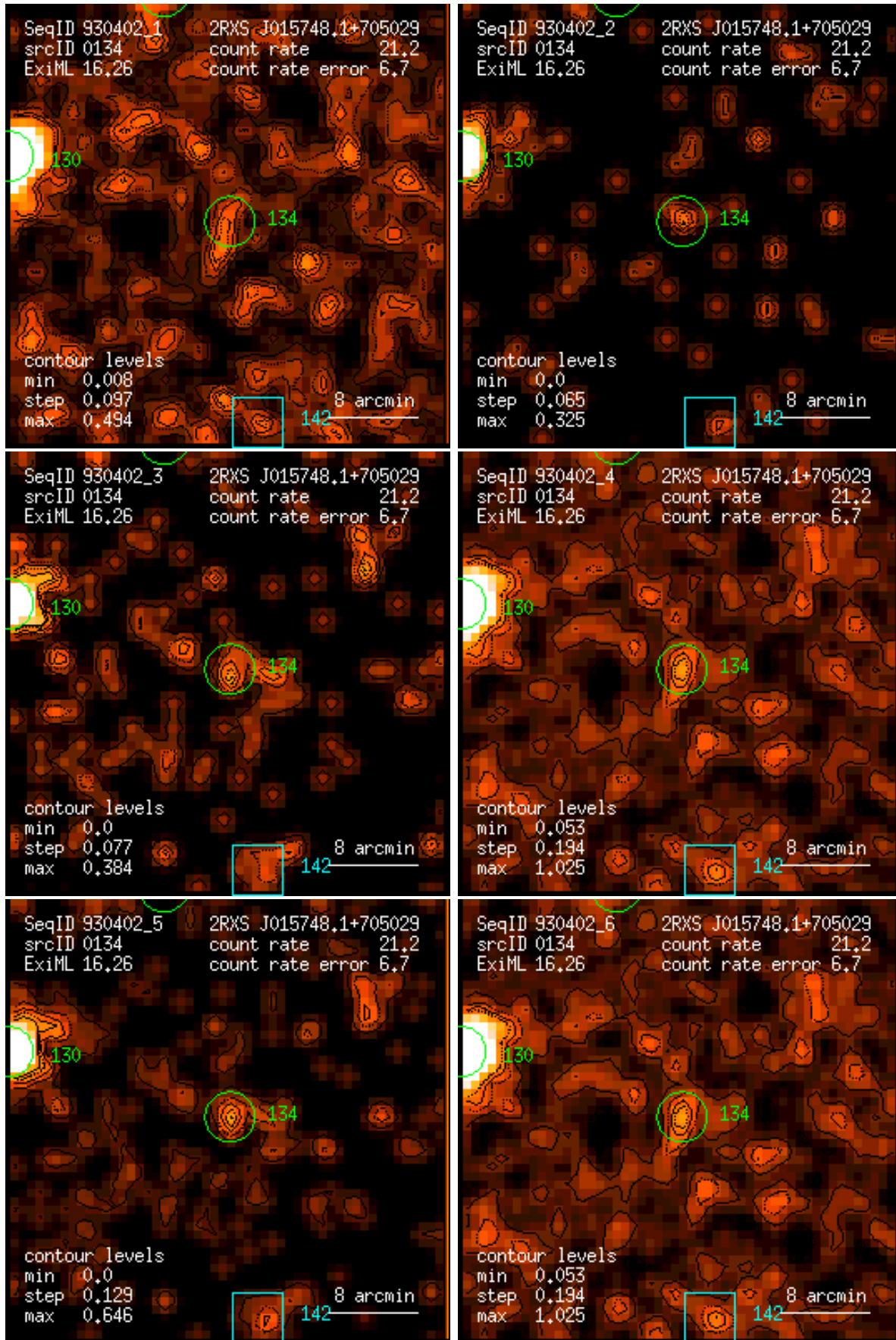
Figure 134: RASS 930402: detection 0134: band rate images, Gaussian filter: (1) PSPC channels 11 – 41, (2) 52 – 90, (3) 91 – 201, (4) 11 – 235, (5) 52 – 201, (6) 11 – 201. Broad band rates in counts/ks. Band rate contour levels in counts/ks/arcmin 2 .
