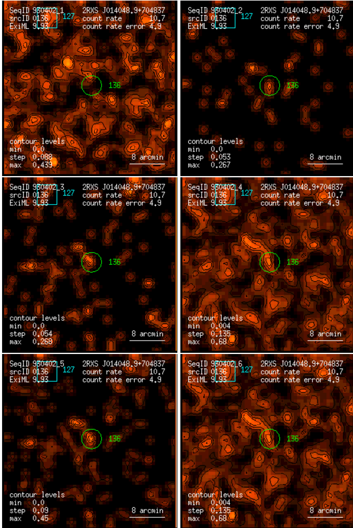
Figure 136: RASS 930402: detection 0136: band rate images, Gaussian filter: (1) PSPC channels 11 – 41, (2) 52 – 90, (3) 91 – 201, (4) 11 – 235, (5) 52 – 201, (6) 11 – 201. Broad band rates in counts/ks. Band rate contour levels in counts/ks/arcmin 2 .
