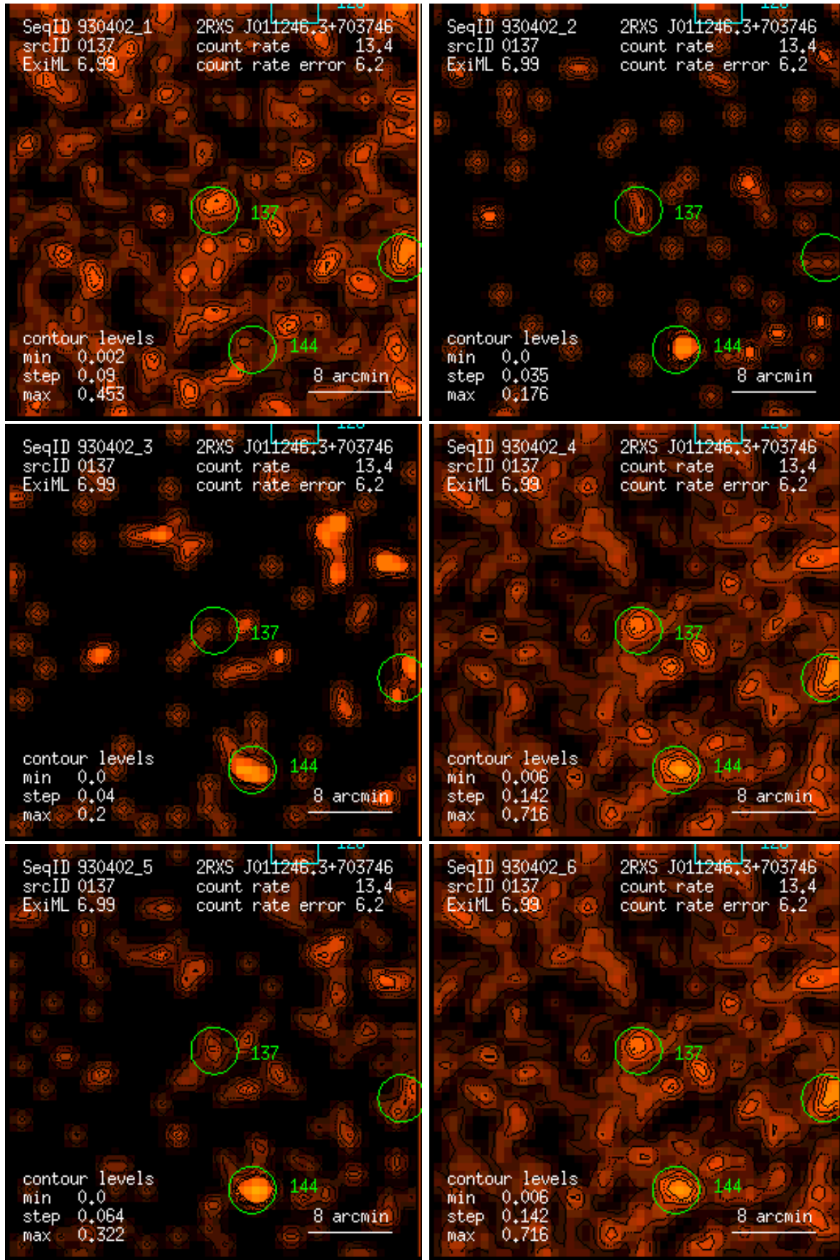
Figure 137: RASS 930402: detection 0137: band rate images, Gaussian filter: (1) PSPC channels 11 – 41, (2) 52 – 90, (3) 91 – 201, (4) 11 – 235, (5) 52 – 201, (6) 11 – 201. Broad band rates in counts/ks. Band rate contour levels in counts/ks/arcmin 2 .
