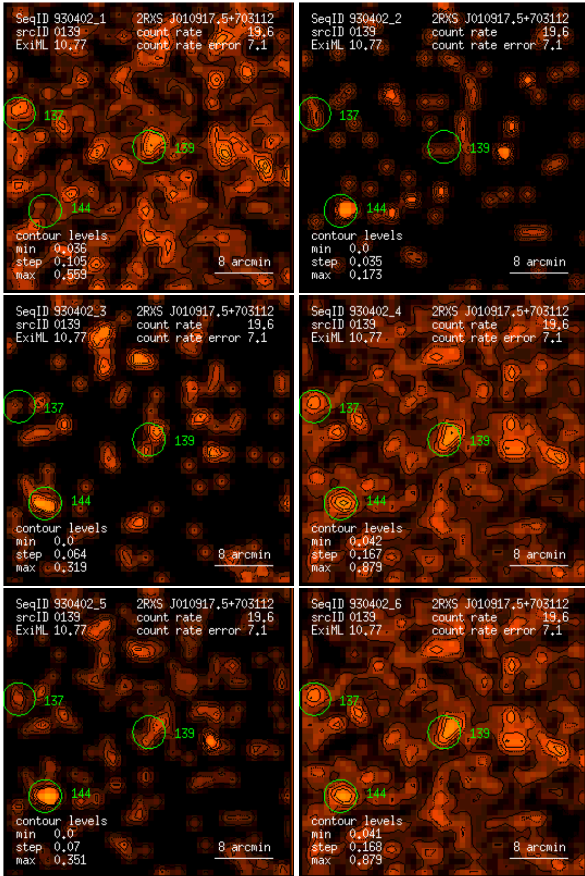
Figure 139: RASS 930402: detection 0139: band rate images, Gaussian filter: (1) PSPC channels 11 – 41, (2) 52 – 90, (3) 91 – 201, (4) 11 – 235, (5) 52 – 201, (6) 11 – 201. Broad band rates in counts/ks. Band rate contour levels in counts/ks/arcmin 2 .
