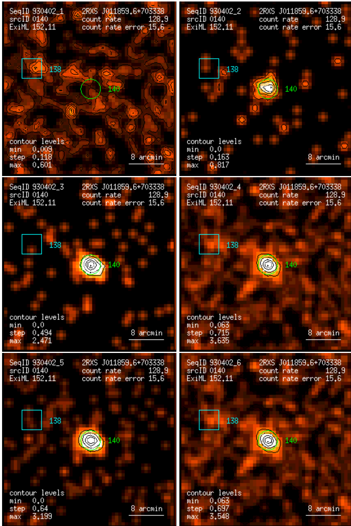
Figure 140: RASS 930402: detection 0140: band rate images, Gaussian filter: (1) PSPC channels 11 – 41, (2) 52 – 90, (3) 91 – 201, (4) 11 – 235, (5) 52 – 201, (6) 11 – 201. Broad band rates in counts/ks. Band rate contour levels in counts/ks/arcmin 2 .
