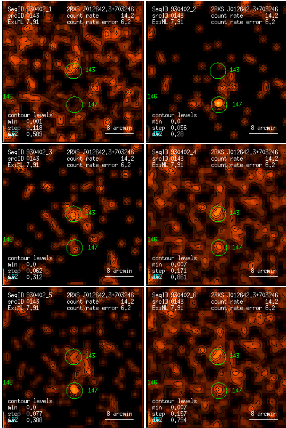
Figure 143: RASS 930402: detection 0143: band rate images, Gaussian filter: (1) PSPC channels 11 – 41, (2) 52 – 90, (3) 91 – 201, (4) 11 – 235, (5) 52 – 201, (6) 11 – 201. Broad band rates in counts/ks. Band rate contour levels in counts/ks/arcmin 2 .
