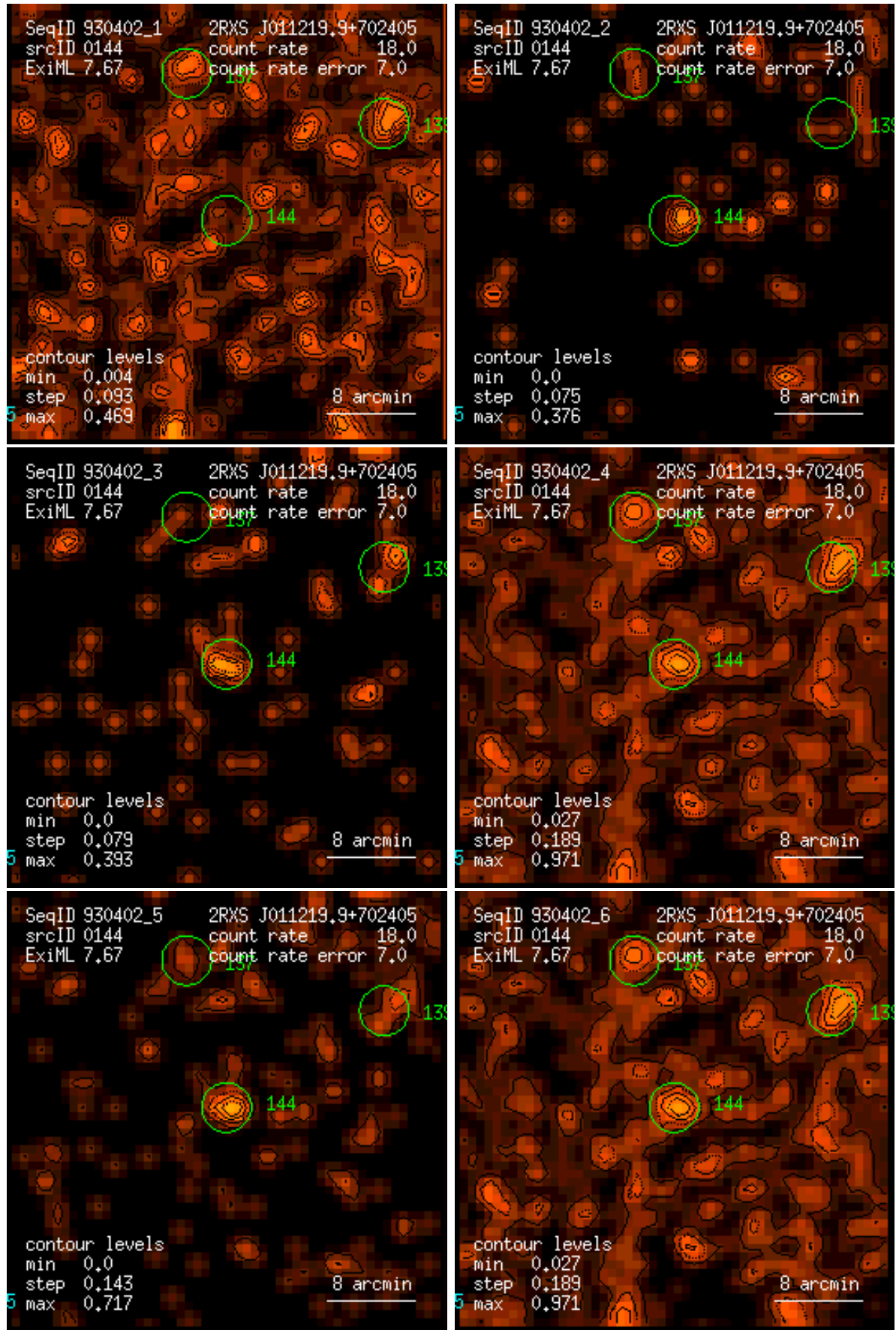
Figure 144: RASS 930402: detection 0144: band rate images, Gaussian filter: (1) PSPC channels 11 – 41, (2) 52 – 90, (3) 91 – 201, (4) 11 – 235, (5) 52 – 201, (6) 11 – 201. Broad band rates in counts/ks. Band rate contour levels in counts/ks/arcmin 2 .
