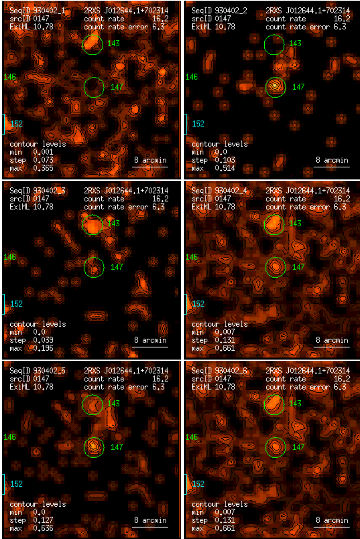
Figure 147: RASS 930402: detection 0147: band rate images, Gaussian filter: (1) PSPC channels 11 – 41, (2) 52 – 90, (3) 91 – 201, (4) 11 – 235, (5) 52 – 201, (6) 11 – 201. Broad band rates in counts/ks. Band rate contour levels in counts/ks/arcmin 2 .
