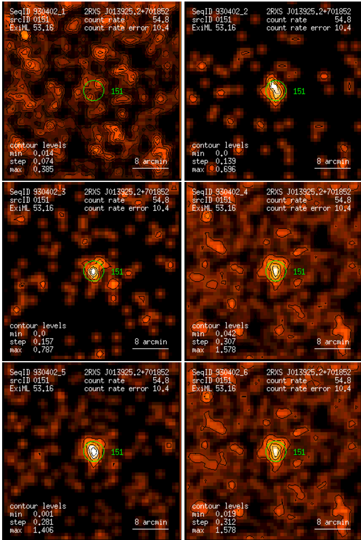
Figure 151: RASS 930402: detection 0151: band rate images, Gaussian filter: (1) PSPC channels 11 – 41, (2) 52 – 90, (3) 91 – 201, (4) 11 – 235, (5) 52 – 201, (6) 11 – 201. Broad band rates in counts/ks. Band rate contour levels in counts/ks/arcmin 2 .
