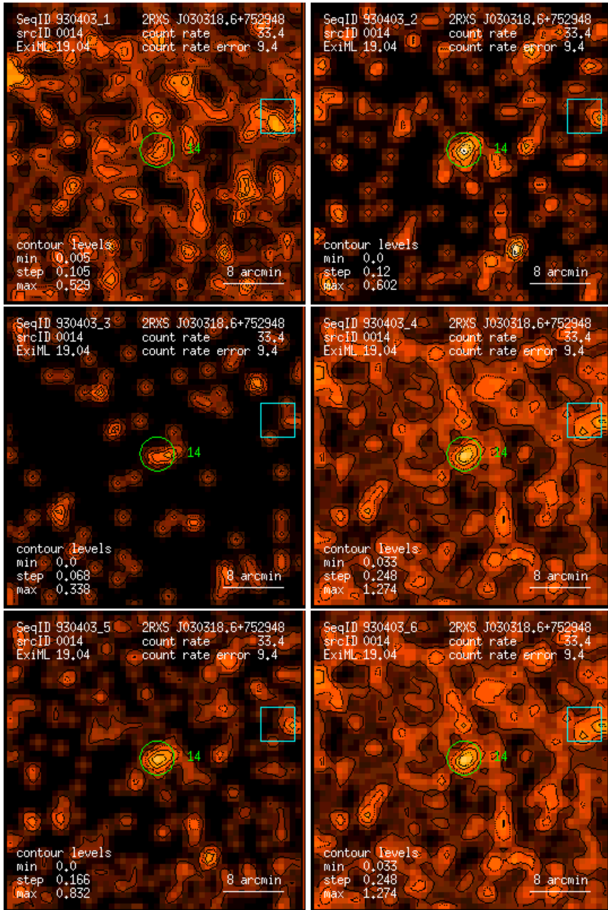
Figure 14: RASS 930403: detection 0014: band rate images, Gaussian filter: (1) PSPC channels 11 – 41, (2) 52 – 90, (3) 91 – 201, (4) 11 – 235, (5) 52 – 201, (6) 11 – 201. Broad band rates in counts/ks. Band rate contour levels in counts/ks/arcmin 2 .
