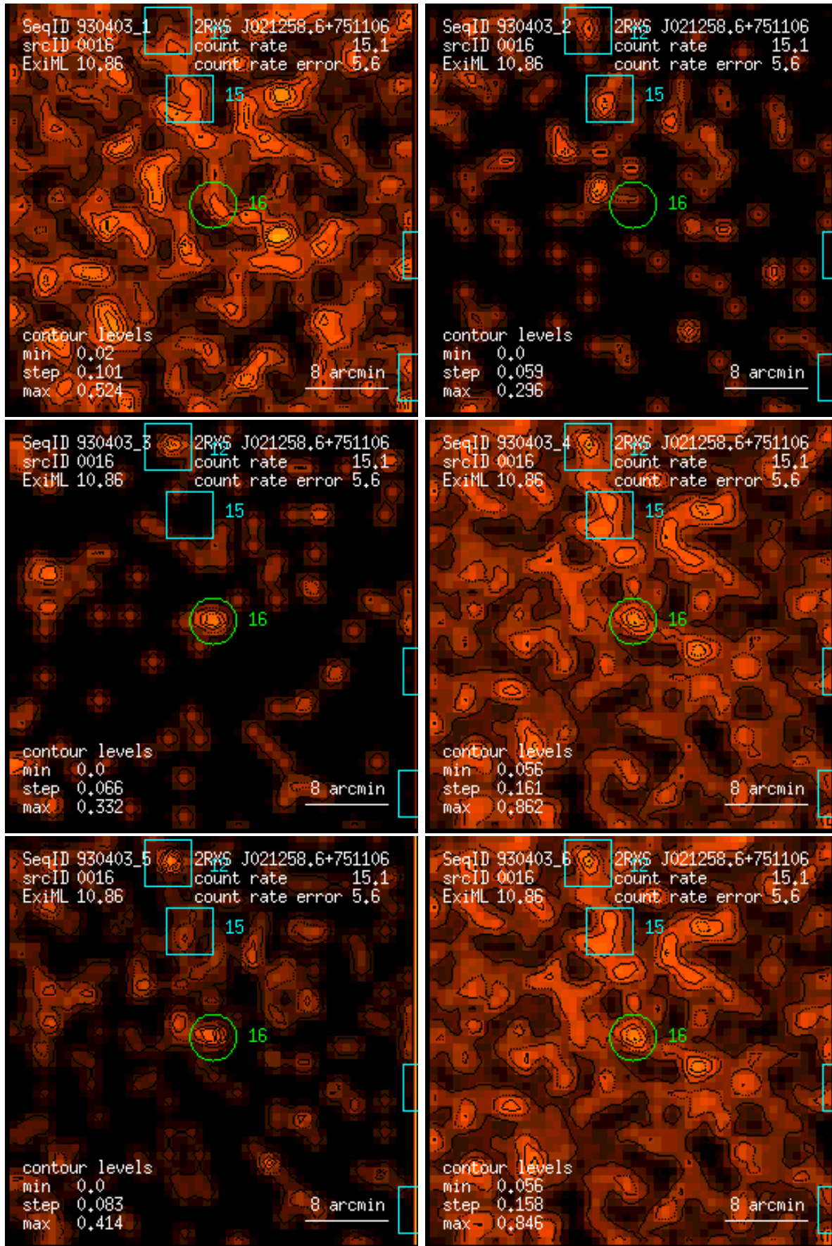
Figure 16: RASS 930403: detection 0016: band rate images, Gaussian filter: (1) PSPC channels 11 – 41, (2) 52 – 90, (3) 91 – 201, (4) 11 – 235, (5) 52 – 201, (6) 11 – 201. Broad band rates in counts/ks. Band rate contour levels in counts/ks/arcmin 2 .
