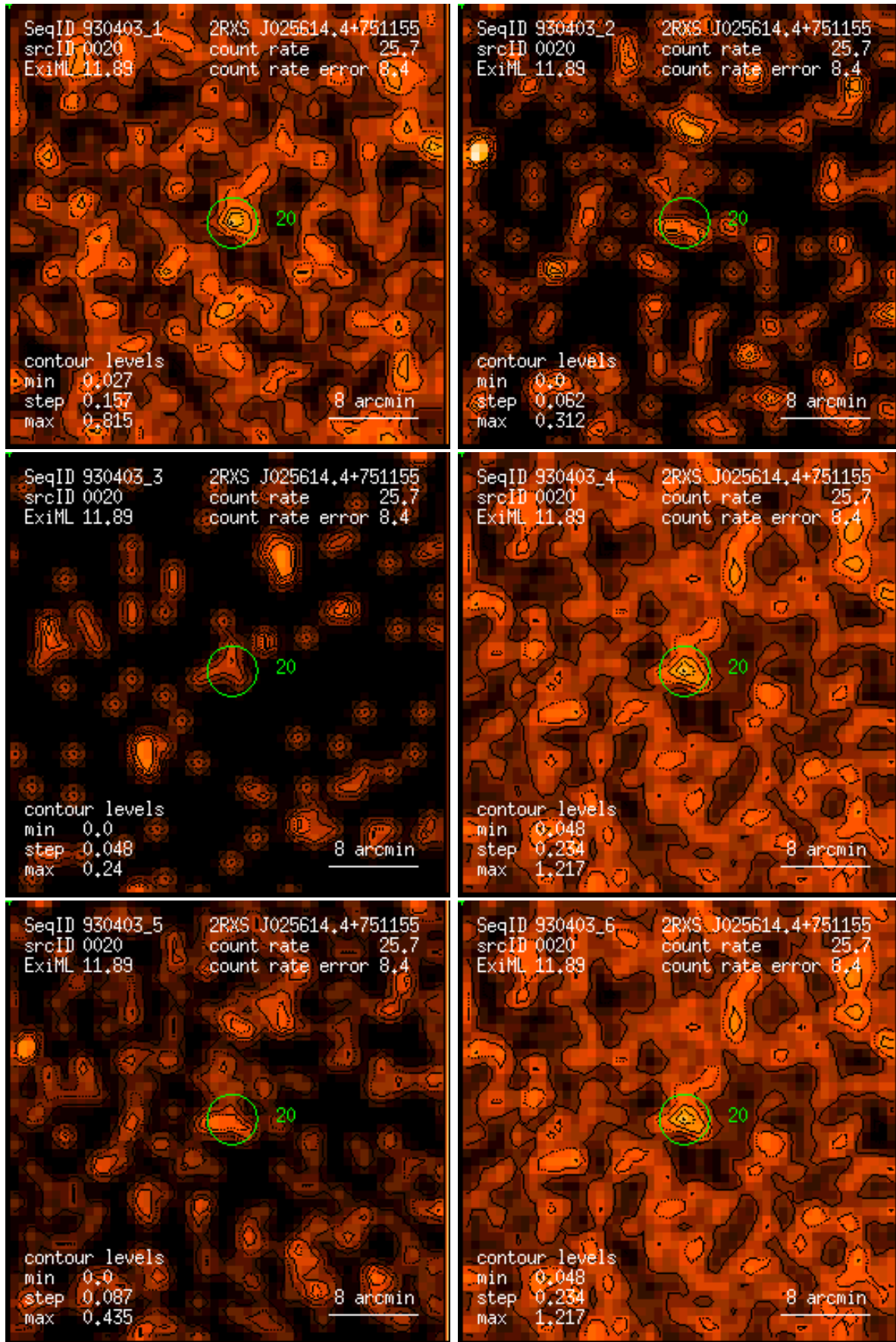
Figure 20: RASS 930403: detection 0020: band rate images, Gaussian filter: (1) PSPC channels 11 – 41, (2) 52 – 90, (3) 91 – 201, (4) 11 – 235, (5) 52 – 201, (6) 11 – 201. Broad band rates in counts/ks. Band rate contour levels in counts/ks/arcmin 2 .
