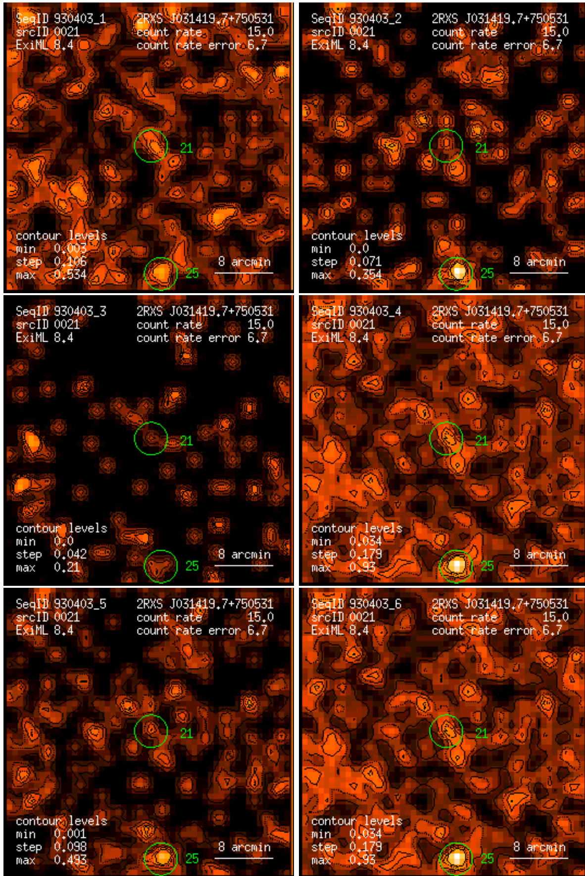
Figure 21: RASS 930403: detection 0021: band rate images, Gaussian filter: (1) PSPC channels 11 – 41, (2) 52 – 90, (3) 91 – 201, (4) 11 – 235, (5) 52 – 201, (6) 11 – 201. Broad band rates in counts/ks. Band rate contour levels in counts/ks/arcmin 2 .
