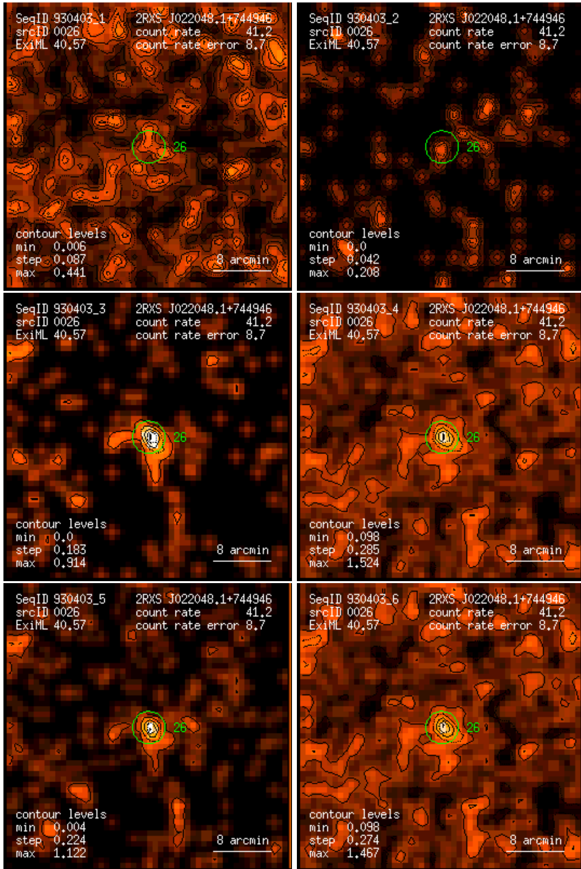
Figure 26: RASS 930403: detection 0026: band rate images, Gaussian filter: (1) PSPC channels 11 – 41, (2) 52 – 90, (3) 91 – 201, (4) 11 – 235, (5) 52 – 201, (6) 11 – 201. Broad band rates in counts/ks. Band rate contour levels in counts/ks/arcmin 2 .
