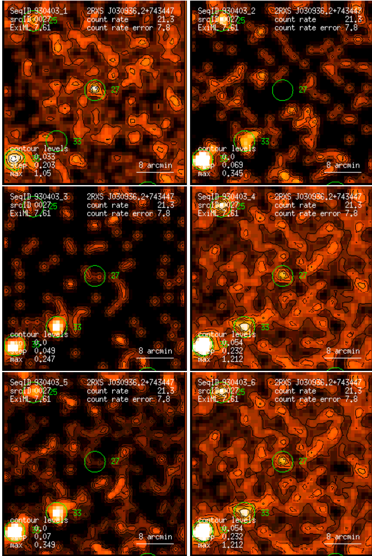
Figure 27: RASS 930403: detection 0027: band rate images, Gaussian filter: (1) PSPC channels 11 – 41, (2) 52 – 90, (3) 91 – 201, (4) 11 – 235, (5) 52 – 201, (6) 11 – 201. Broad band rates in counts/ks. Band rate contour levels in counts/ks/arcmin 2 .
