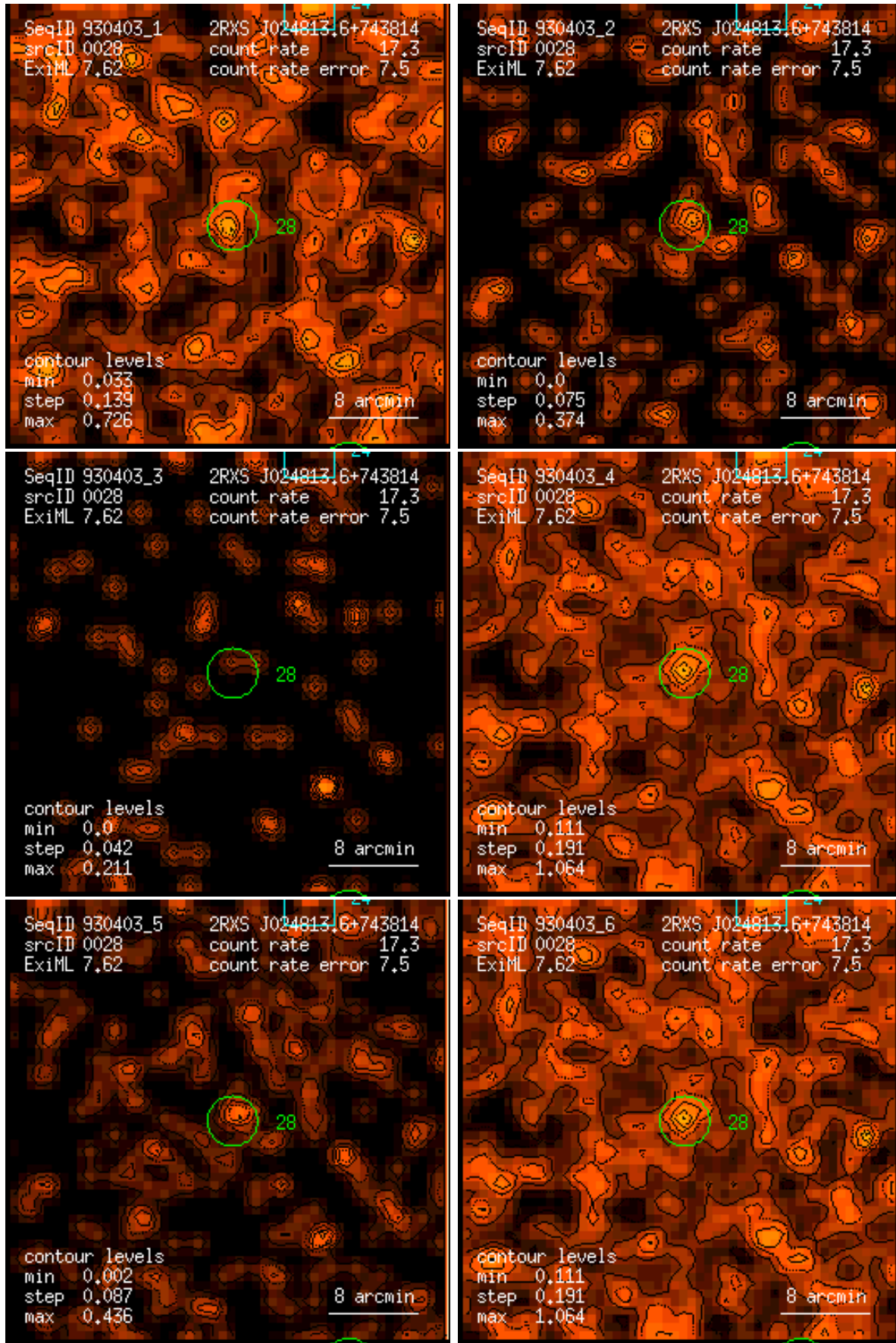
Figure 28: RASS 930403: detection 0028: band rate images, Gaussian filter: (1) PSPC channels 11 – 41, (2) 52 – 90, (3) 91 – 201, (4) 11 – 235, (5) 52 – 201, (6) 11 – 201. Broad band rates in counts/ks. Band rate contour levels in counts/ks/arcmin 2 .
