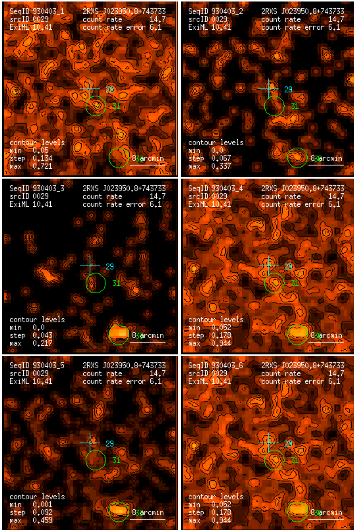
Figure 29: RASS 930403: detection 0029: band rate images, Gaussian filter: (1) PSPC channels 11 – 41, (2) 52 – 90, (3) 91 – 201, (4) 11 – 235, (5) 52 – 201, (6) 11 – 201. Broad band rates in counts/ks. Band rate contour levels in counts/ks/arcmin 2 .
