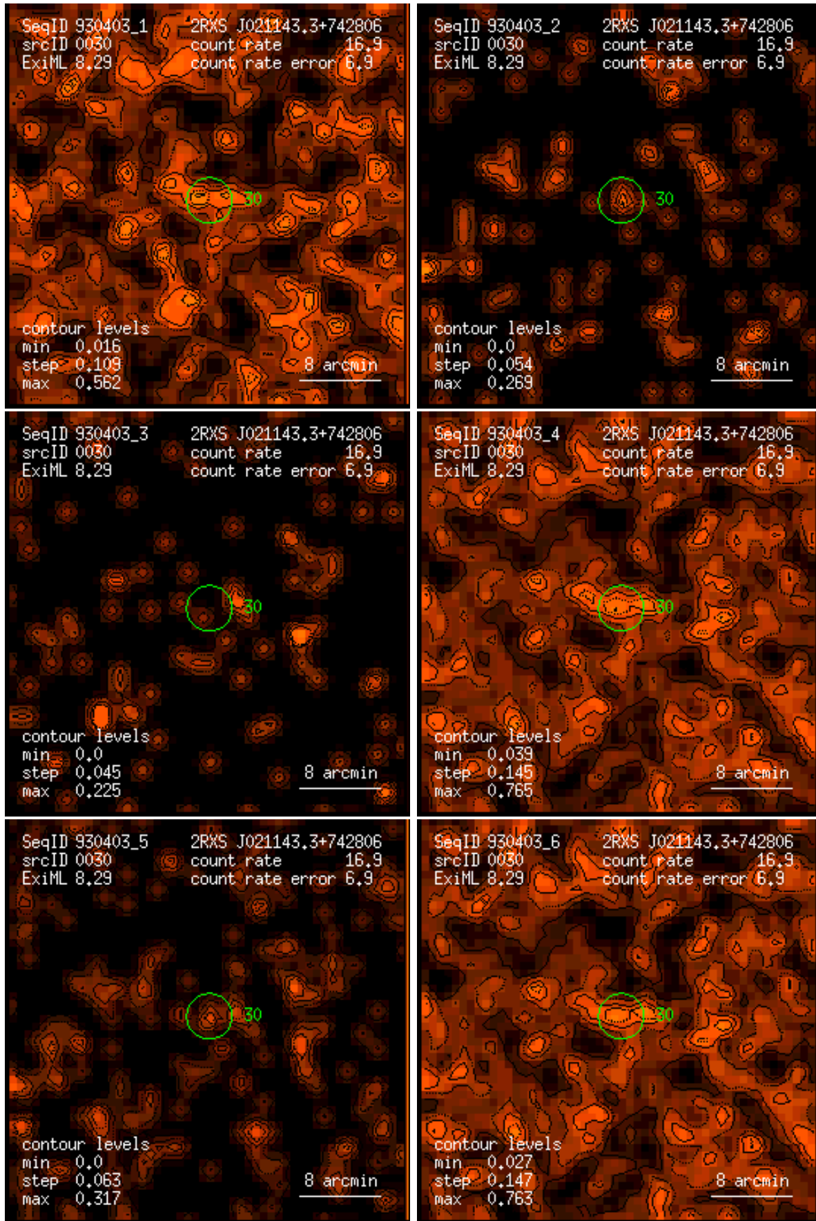
Figure 30: RASS 930403: detection 0030: band rate images, Gaussian filter: (1) PSPC channels 11 – 41, (2) 52 – 90, (3) 91 – 201, (4) 11 – 235, (5) 52 – 201, (6) 11 – 201. Broad band rates in counts/ks. Band rate contour levels in counts/ks/arcmin 2 .
