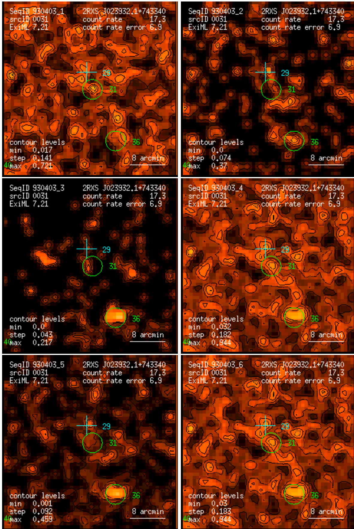
Figure 31: RASS 930403: detection 0031: band rate images, Gaussian filter: (1) PSPC channels 11 – 41, (2) 52 – 90, (3) 91 – 201, (4) 11 – 235, (5) 52 – 201, (6) 11 – 201. Broad band rates in counts/ks. Band rate contour levels in counts/ks/arcmin 2 .
