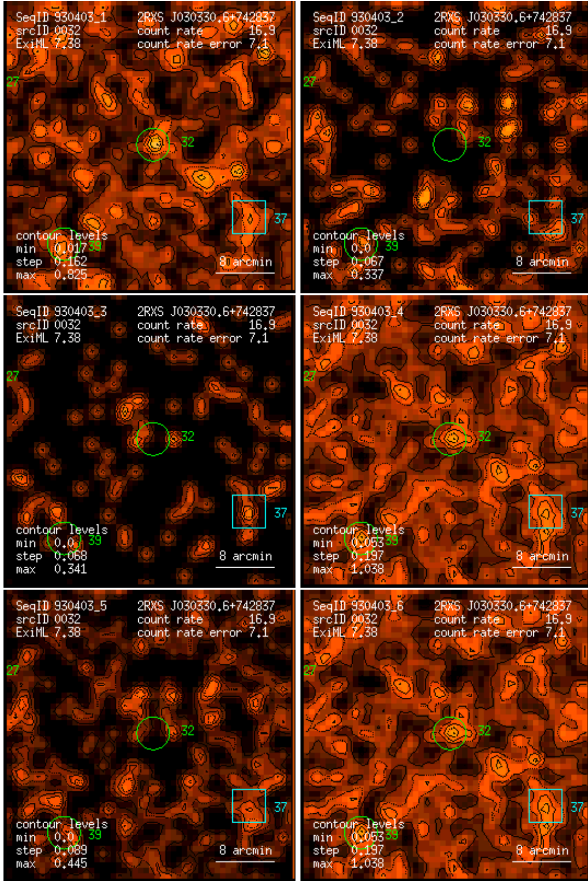
Figure 32: RASS 930403: detection 0032: band rate images, Gaussian filter: (1) PSPC channels 11 – 41, (2) 52 – 90, (3) 91 – 201, (4) 11 – 235, (5) 52 – 201, (6) 11 – 201. Broad band rates in counts/ks. Band rate contour levels in counts/ks/arcmin 2 .
