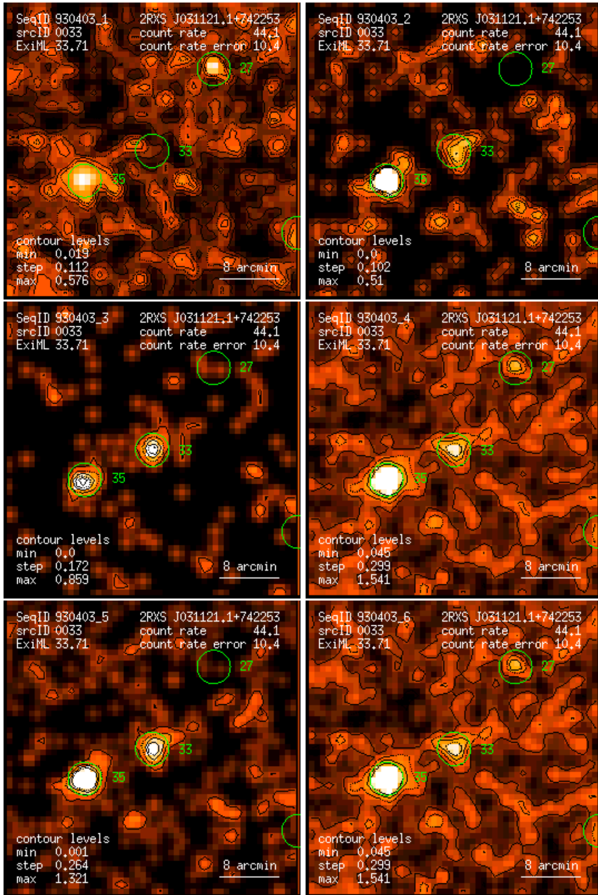
Figure 33: RASS 930403: detection 0033: band rate images, Gaussian filter: (1) PSPC channels 11 – 41, (2) 52 – 90, (3) 91 – 201, (4) 11 – 235, (5) 52 – 201, (6) 11 – 201. Broad band rates in counts/ks. Band rate contour levels in counts/ks/arcmin 2 .
