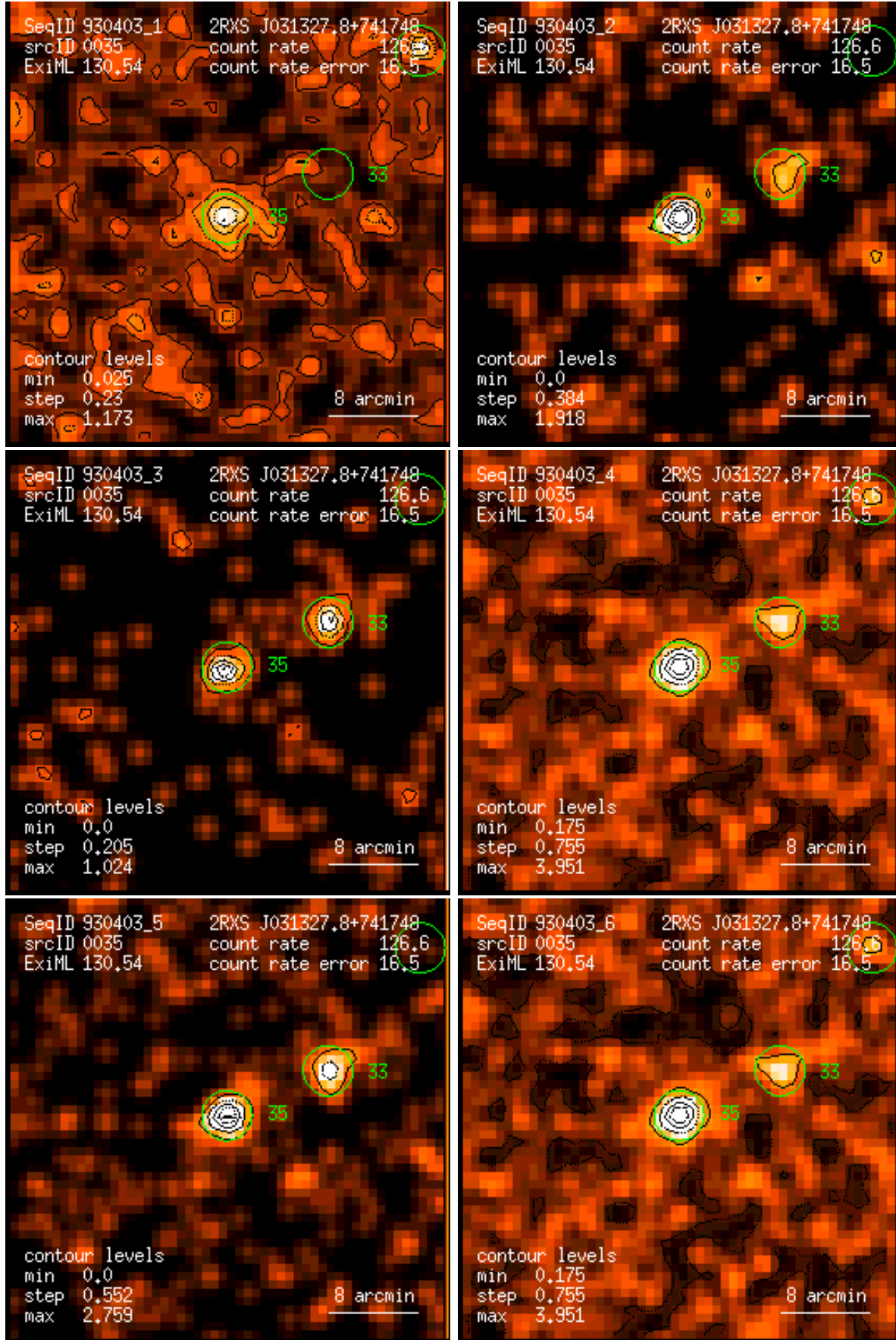
Figure 35: RASS 930403: detection 0035: band rate images, Gaussian filter: (1) PSPC channels 11 – 41, (2) 52 – 90, (3) 91 – 201, (4) 11 – 235, (5) 52 – 201, (6) 11 – 201. Broad band rates in counts/ks. Band rate contour levels in counts/ks/arcmin 2 .
