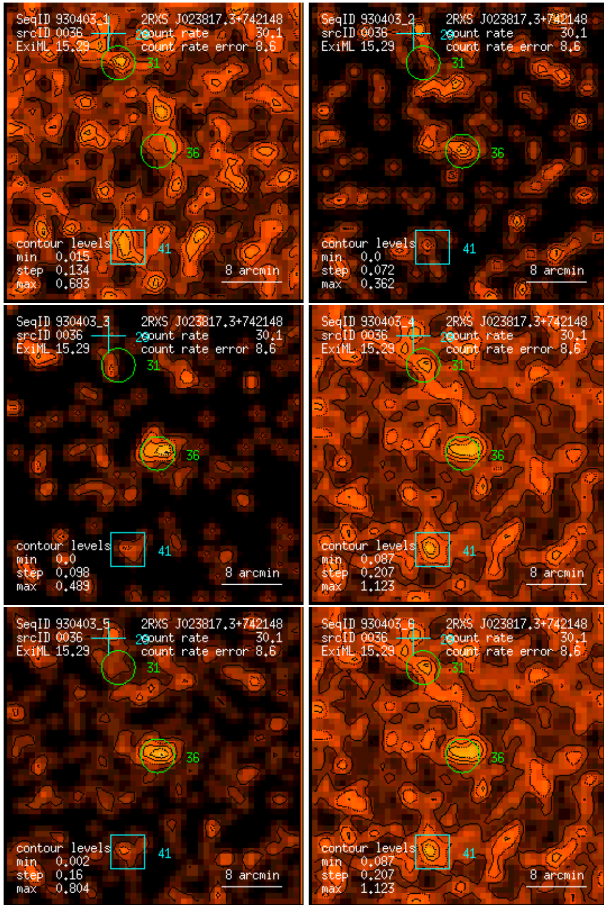
Figure 36: RASS 930403: detection 0036: band rate images, Gaussian filter: (1) PSPC channels 11 – 41, (2) 52 – 90, (3) 91 – 201, (4) 11 – 235, (5) 52 – 201, (6) 11 – 201. Broad band rates in counts/ks. Band rate contour levels in counts/ks/arcmin 2 .
