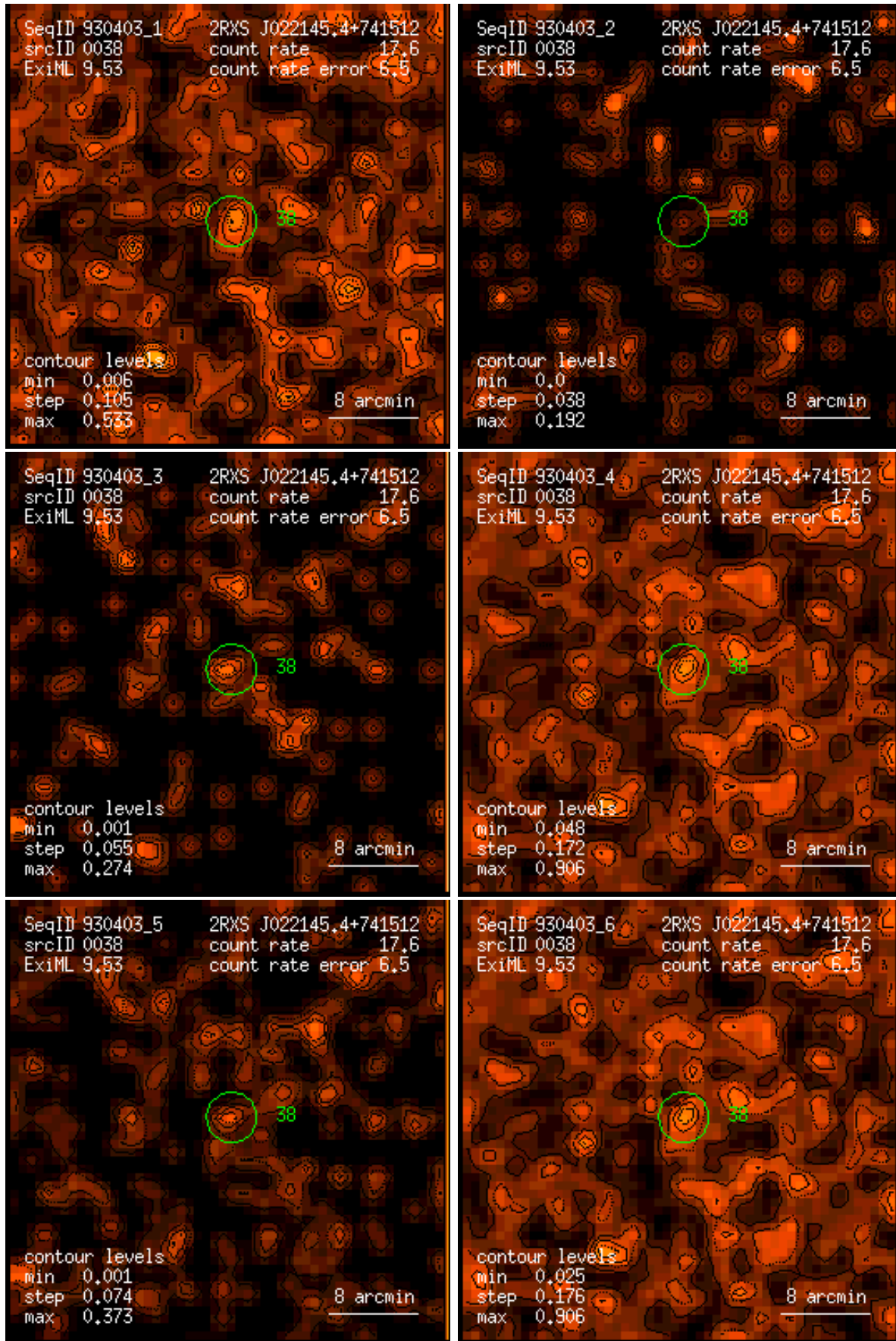
Figure 38: RASS 930403: detection 0038: band rate images, Gaussian filter: (1) PSPC channels 11 – 41, (2) 52 – 90, (3) 91 – 201, (4) 11 – 235, (5) 52 – 201, (6) 11 – 201. Broad band rates in counts/ks. Band rate contour levels in counts/ks/arcmin 2 .
