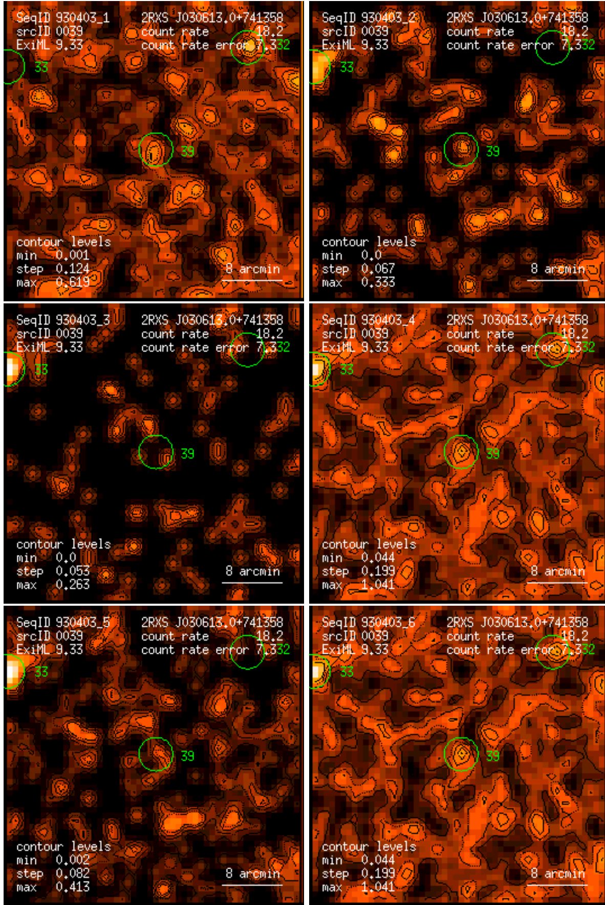
Figure 39: RASS 930403: detection 0039: band rate images, Gaussian filter: (1) PSPC channels 11 – 41, (2) 52 – 90, (3) 91 – 201, (4) 11 – 235, (5) 52 – 201, (6) 11 – 201. Broad band rates in counts/ks. Band rate contour levels in counts/ks/arcmin 2 .
