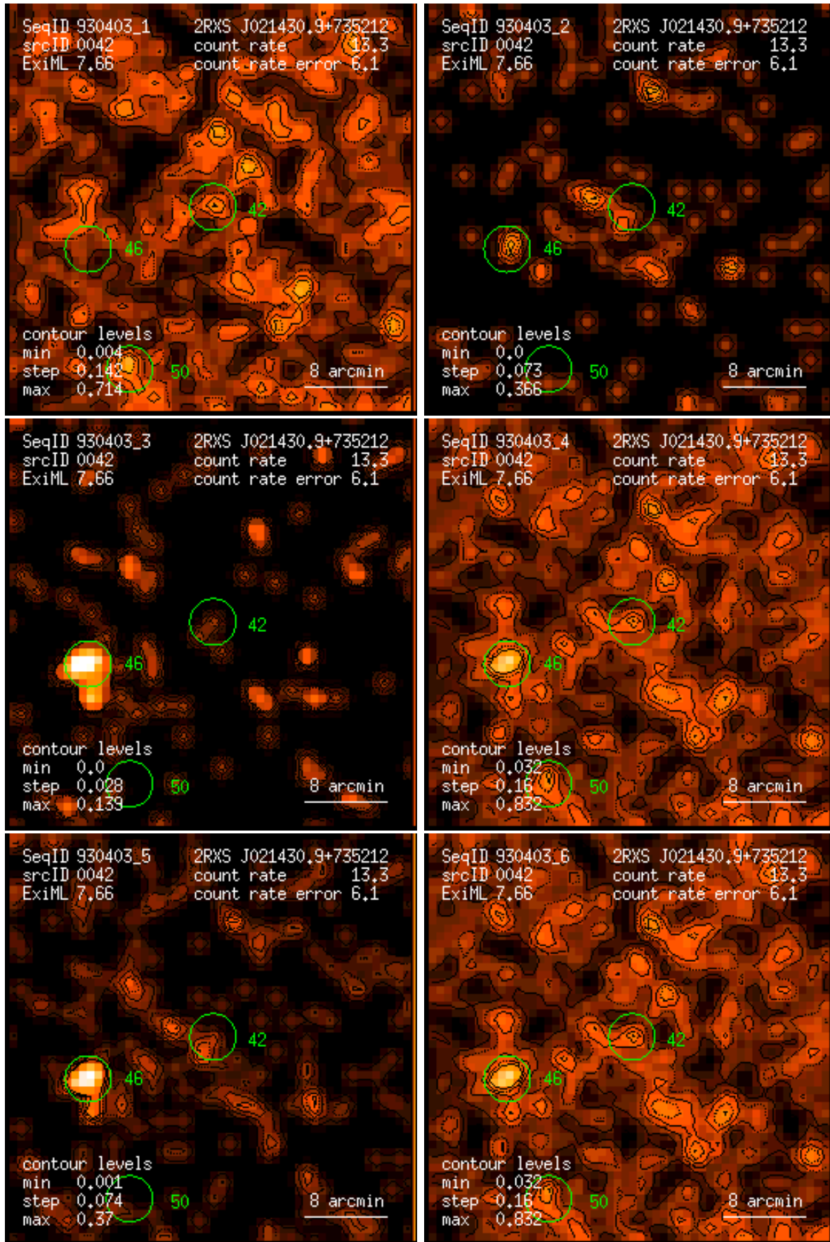
Figure 42: RASS 930403: detection 0042: band rate images, Gaussian filter: (1) PSPC channels 11 – 41, (2) 52 – 90, (3) 91 – 201, (4) 11 – 235, (5) 52 – 201, (6) 11 – 201. Broad band rates in counts/ks. Band rate contour levels in counts/ks/arcmin 2 .
