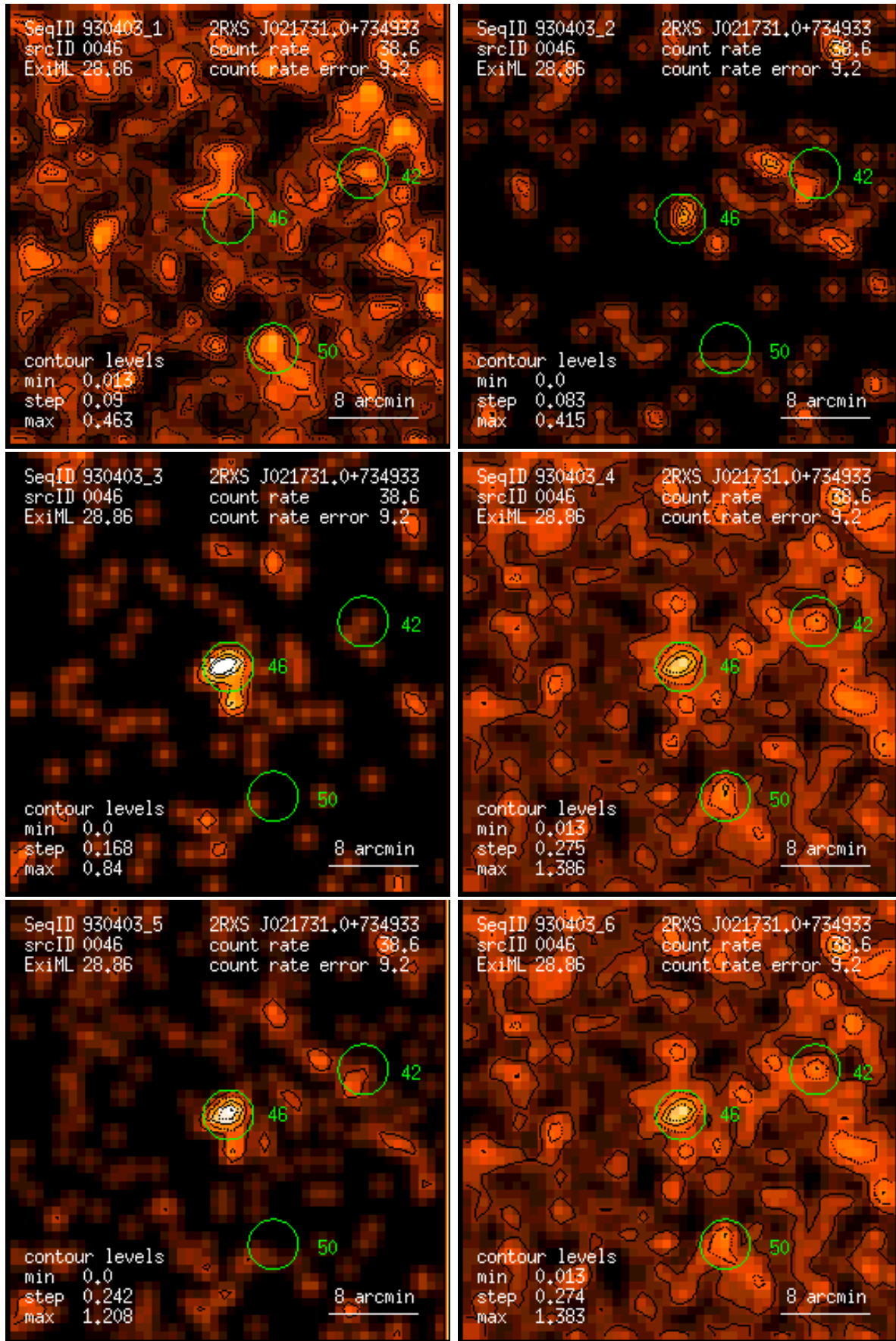
Figure 46: RASS 930403: detection 0046: band rate images, Gaussian filter: (1) PSPC channels 11 – 41, (2) 52 – 90, (3) 91 – 201, (4) 11 – 235, (5) 52 – 201, (6) 11 – 201. Broad band rates in counts/ks. Band rate contour levels in counts/ks/arcmin 2 .
