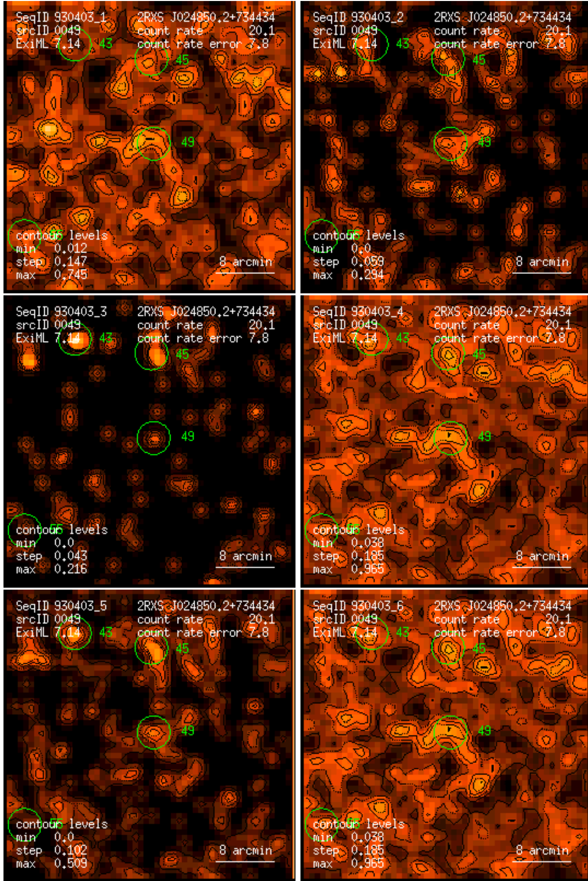
Figure 49: RASS 930403: detection 0049: band rate images, Gaussian filter: (1) PSPC channels 11 – 41, (2) 52 – 90, (3) 91 – 201, (4) 11 – 235, (5) 52 – 201, (6) 11 – 201. Broad band rates in counts/ks. Band rate contour levels in counts/ks/arcmin 2 .
