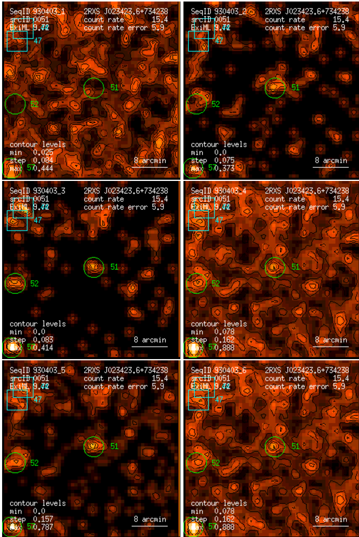
Figure 51: RASS 930403: detection 0051: band rate images, Gaussian filter: (1) PSPC channels 11 – 41, (2) 52 – 90, (3) 91 – 201, (4) 11 – 235, (5) 52 – 201, (6) 11 – 201. Broad band rates in counts/ks. Band rate contour levels in counts/ks/arcmin 2 .
