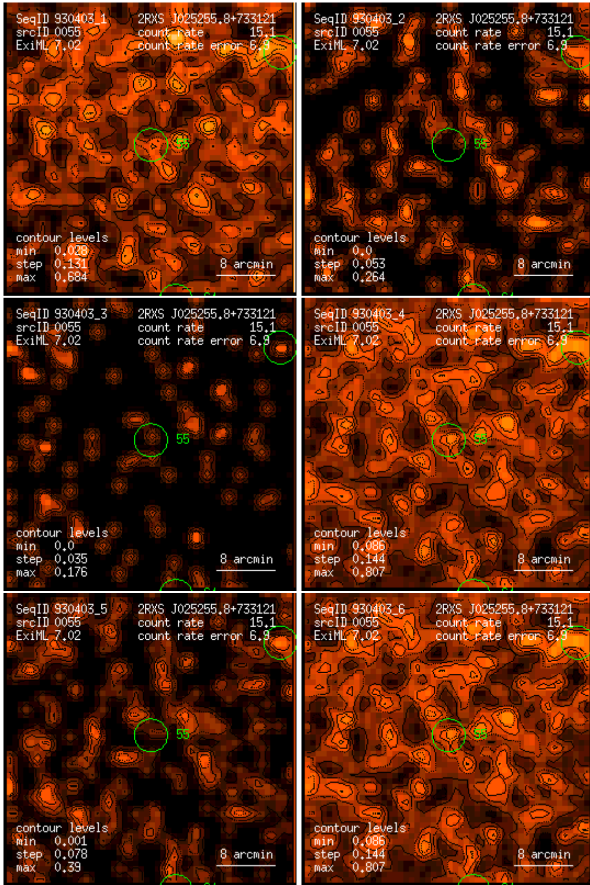
Figure 55: RASS 930403: detection 0055: band rate images, Gaussian filter: (1) PSPC channels 11 – 41, (2) 52 – 90, (3) 91 – 201, (4) 11 – 235, (5) 52 – 201, (6) 11 – 201. Broad band rates in counts/ks. Band rate contour levels in counts/ks/arcmin 2 .
