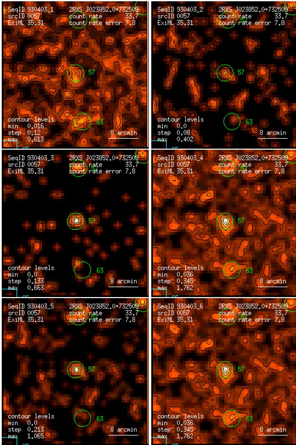
Figure 57: RASS 930403: detection 0057: band rate images, Gaussian filter: (1) PSPC channels 11 – 41, (2) 52 – 90, (3) 91 – 201, (4) 11 – 235, (5) 52 – 201, (6) 11 – 201. Broad band rates in counts/ks. Band rate contour levels in counts/ks/arcmin 2 .
