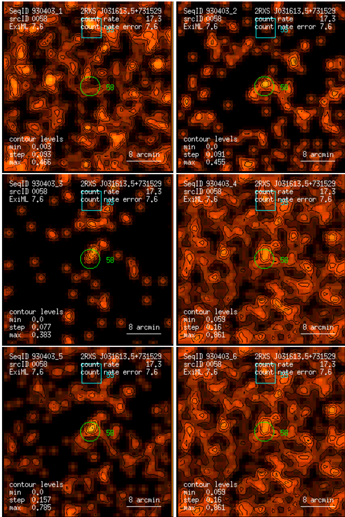
Figure 58: RASS 930403: detection 0058: band rate images, Gaussian filter: (1) PSPC channels 11 – 41, (2) 52 – 90, (3) 91 – 201, (4) 11 – 235, (5) 52 – 201, (6) 11 – 201. Broad band rates in counts/ks. Band rate contour levels in counts/ks/arcmin 2 .
