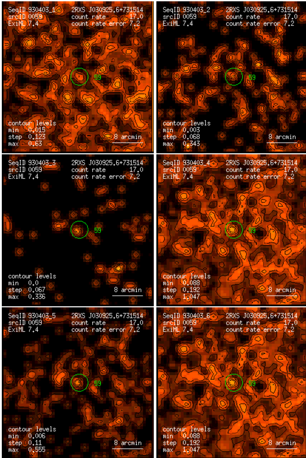
Figure 59: RASS 930403: detection 0059: band rate images, Gaussian filter: (1) PSPC channels 11 – 41, (2) 52 – 90, (3) 91 – 201, (4) 11 – 235, (5) 52 – 201, (6) 11 – 201. Broad band rates in counts/ks. Band rate contour levels in counts/ks/arcmin 2 .
