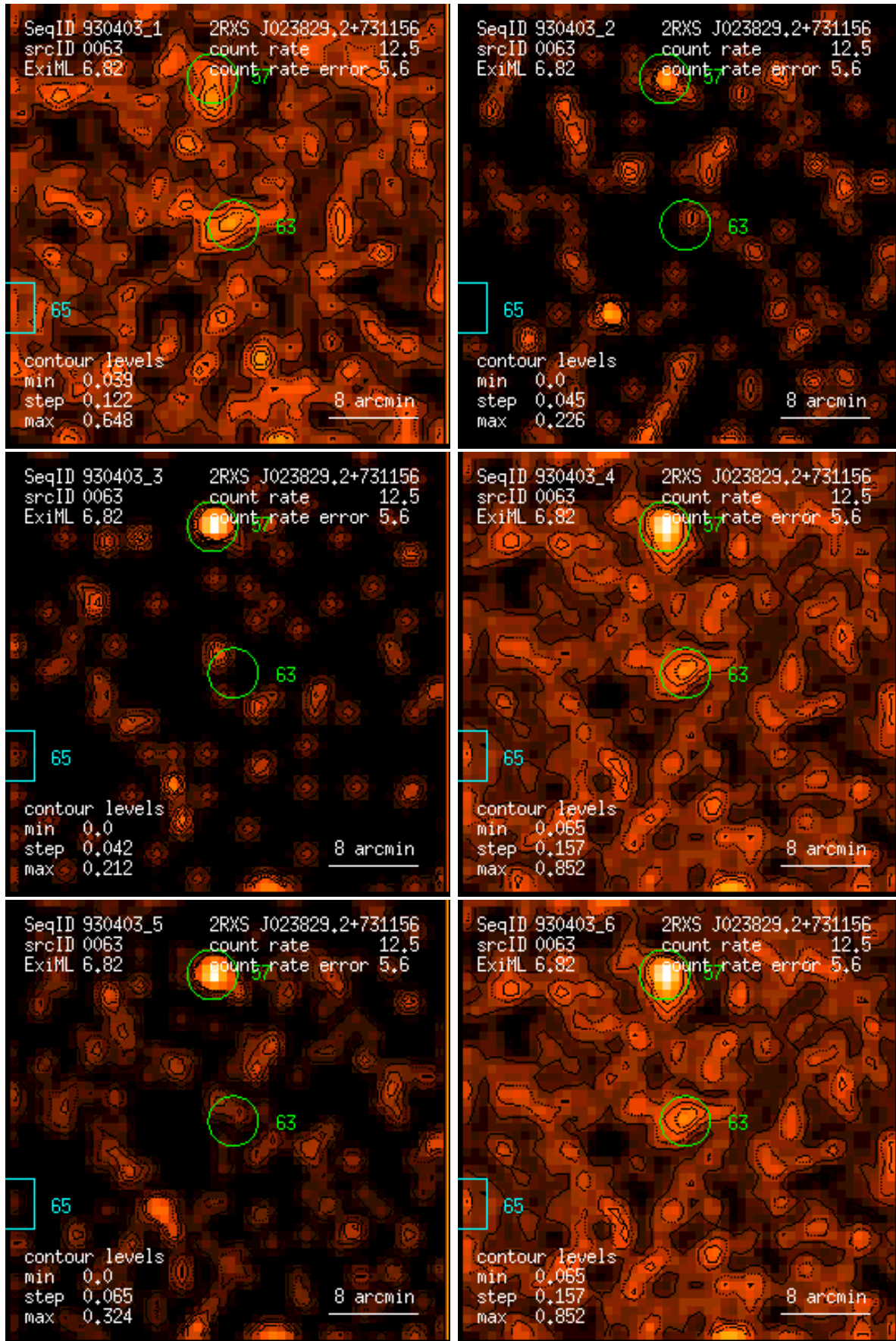
Figure 63: RASS 930403: detection 0063: band rate images, Gaussian filter: (1) PSPC channels 11 – 41, (2) 52 – 90, (3) 91 – 201, (4) 11 – 235, (5) 52 – 201, (6) 11 – 201. Broad band rates in counts/ks. Band rate contour levels in counts/ks/arcmin 2 .
