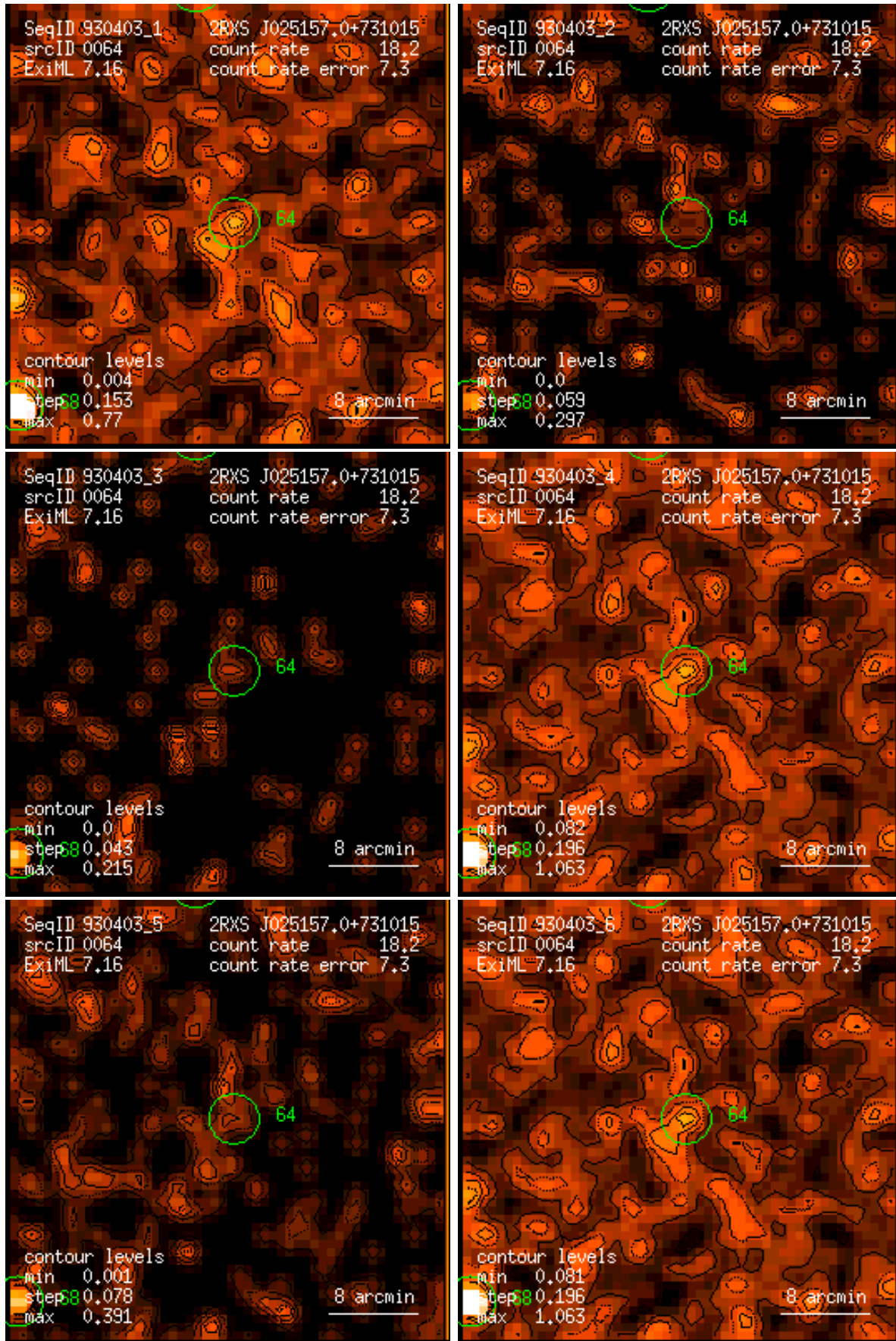
Figure 64: RASS 930403: detection 0064: band rate images, Gaussian filter: (1) PSPC channels 11 – 41, (2) 52 – 90, (3) 91 – 201, (4) 11 – 235, (5) 52 – 201, (6) 11 – 201. Broad band rates in counts/ks. Band rate contour levels in counts/ks/arcmin 2 .
